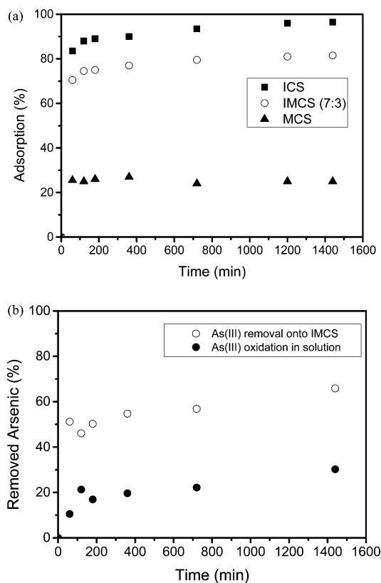
Figure 7. Adsorption of (a) phosphate onto ICS, IMCS(7:3), and MCS at pH 4.5 and (b) arsenic onto IMCS(7:3) at pH 6.5 as a function of time.
