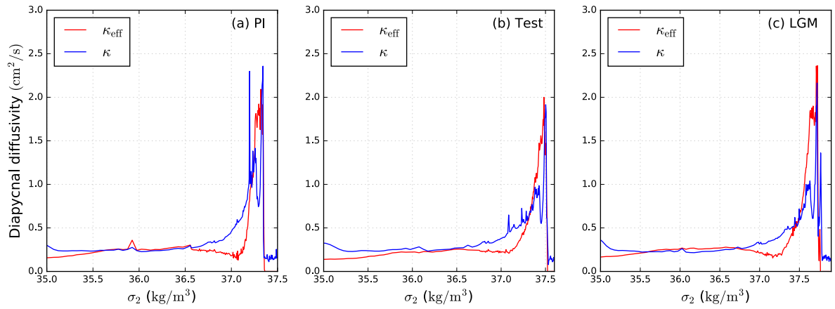
Figure S13. Effective diapycnal diffusivity ( \kappa_{\text{eff}} , defined in Equation (S4)) and model-reported diapycnal diffusivity ( \kappa , defined in Equation (S5)) calculated between 30°S and 30°N. The potential density range covers the depth range from intermediate depth to the ocean bottom.
