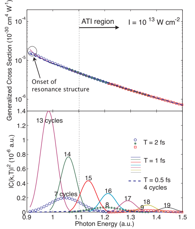
FIG. 5: (Color online) Top panel: two-photon generalized cross sections in the ATI region calculated with pulses of 0.5, 1 and 2 fs as functions of photon energy. Field linear polarization parallel to molecular axis. Lower panel: Squared amplitudes in atomic units, from which the cross sections in the top panel were calculated.
