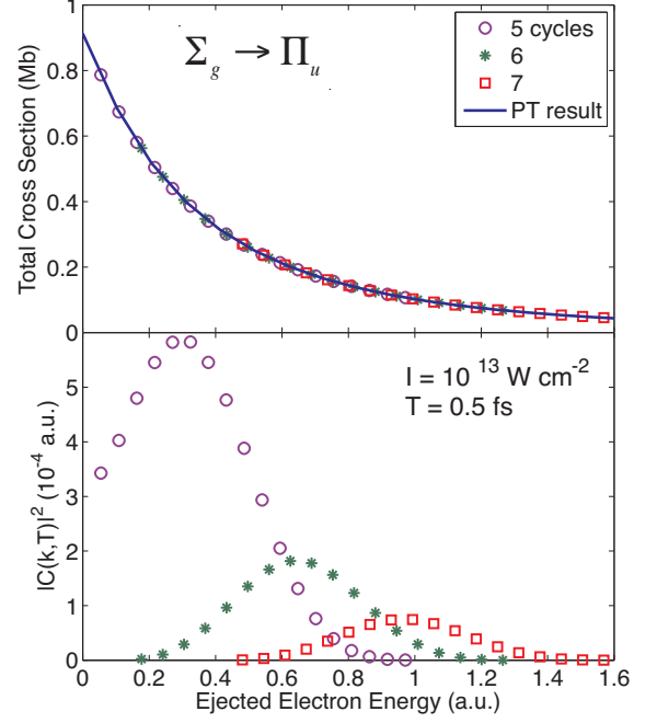
FIG. 3: (Color online) As in Fig. 2, but with photon polarization perpendicular to the molecular axis, pulse duration T=0.5 \text{ fs} with 5, 6 and 7 cycles.
