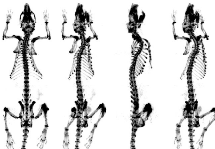
Figure 9. Maximum intensity projection views of bone scan of a 304 g rat injected with 107 MBq (2.9 mCi) of ^{18}\text{F}^- , scanned across five bed positions at 20 min per bed position, starting 210 min after injection. Image reconstructed by MAP with \beta equal to 0 (MLEM).
