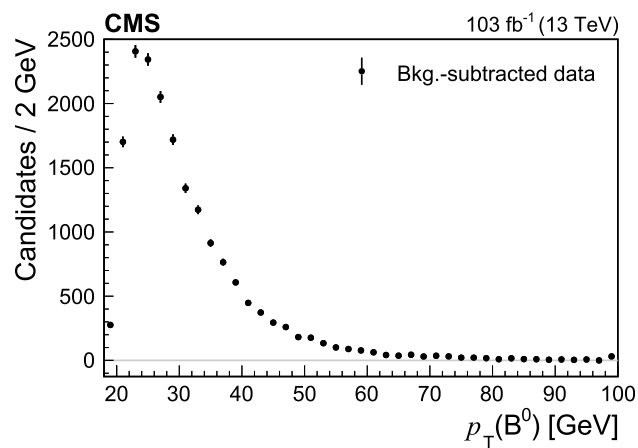
Fig. 4 Background-subtracted p_T(B^0) distribution in data for the B^0 \rightarrow \psi(2S)K_S^0 \pi^+ \pi^- signal. The last bin includes the overflow
