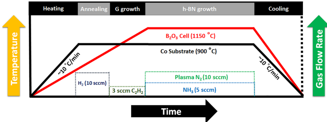
Figure 2.3. Typical growth conditions of h-BN/G heterostructure samples in regions 1-3. To carry out the growth of h-BN/G heterostructure samples, Co substrate was first heated up to 850~950 ^{\circ}\text{C} and annealed for 15 minutes with 10 sccm H 2 gas. Then, the substrate was treated with C (3-sccm C 2 H 2 gas) for a duration of 5 sec~3 min for different samples, and immediately after that, h-BN growth was started. During the h-BN growth, B cell temperature was maintained at 1150 ^{\circ}\text{C} . A mixture of N sources consisting of N 2 gas flowed at 10 sccm through an ECR plasma generator and NH 3 gas leaked at a flow rate of 5 sccm through a needle valve was introduced into the chamber. The h-BN growth lasted from 15 min to 3 hrs for different samples. The substrate heating/cooling rate was \sim 10 ^{\circ}\text{C}/\text{min} for all samples.
