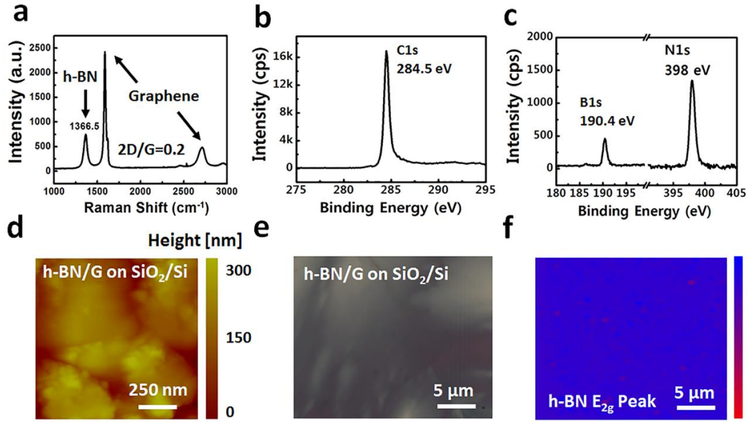
Figure 2.13. Characterization of h-BN/G sample in region 2. (a) Representative Raman spectrum of the as-grown sample. (b) C1s and (c) B1s and N1s XPS signals of the same sample. (d) AFM image of transferred h-BN/G sample with 1.5-min C treatment time onto SiO 2 /Si substrate. (e) OM image of the transferred sample and (f) h-BN E 2g phonon peak intensity mapping of (e).
