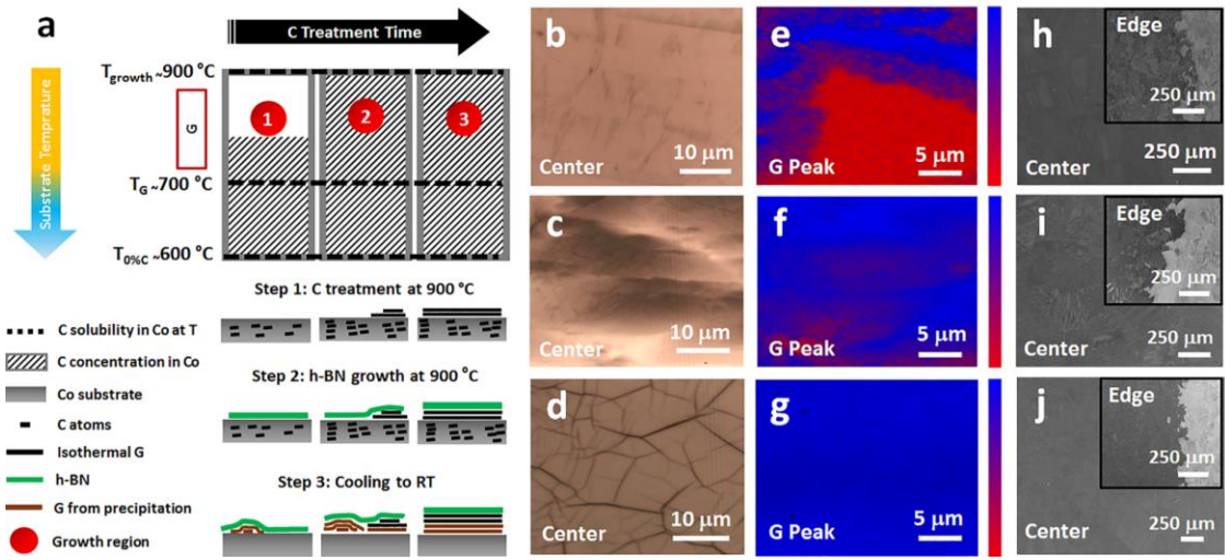
Figure 2.4. H-BN/G heterostructure growth regions on Co substrate. (a) Schematic of h-BN/G growth steps on Co substrate with different C treatment time and same h-BN growth conditions (3 hrs at 900 °C). Three growth regions are identified based on the C treatment time and G growth mode/morphology in h-BN/G samples. (b-d) OM images, (e-g) graphene G peak intensity mapping, and (h-j) SEM images of the samples with 30-sec, 1.5-min, and 3-min C treatment time, which are representative samples in regions 1, 2, and 3, respectively.
