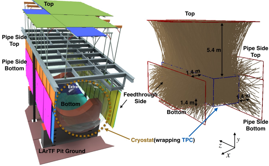
Figure 1: The design of CRT planes as part of the MicroBooNE detector. Simulation of cosmic rays crossing the CRT, the brown lines represent possible cosmic ray trajectories. There are four CRT planes: top plane, bottom plane, pipe side plane and feedthrough side plane. The beam direction is along the z axis.
