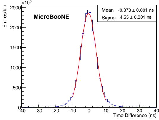
(a) \Delta t for CRT hits in the bottom plane.
