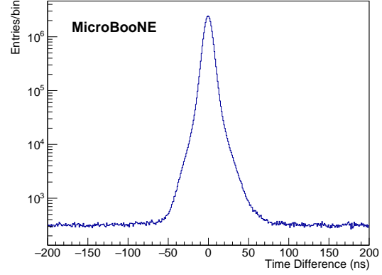
(b) Zoomed-in \Delta t for CRT hits in the bottom plane.
