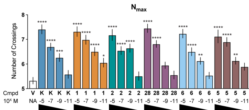
Figure 8. Concentration–response experiments demonstrate that DMTs and isoDMTs have similar psychoplastogenic potencies. The maximum number of crossings ( N_{max} ) of the Sholl plots for cortical neurons treated with compounds at concentrations ranging from 10 \mu\text{M} to 10 \text{ pM} ( n = 66 – 123 neurons). Data are represented as mean \pm SEM. * p < 0.05 , ** p < 0.01 , *** p < 0.001 , **** p < 0.0001 , as compared to the vehicle control following a one-way ANOVA with Dunnett's post hoc test ( F = 15.40 ; DFn = 24 ; DFd = 2,276 ; p -value < 0.0001 ). V = vehicle, K = ketamine.
