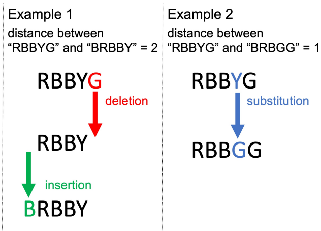
Figure 2. Examples of Levenshtein distance calculations. Example 1: Changing "RBBYG" to "BRBBY" requires one deletion and one insertion, then the distance is two. Example 2: Changing "RBBYG" to "RBBGG" requires only one substitution, then the distance is one.
