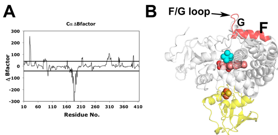
Figure 4. \Delta B factor plot (complex-open) as a function of residue number. For the open state MD trajectories runs of 456, 500, and four 100 ns were merged, whereas for P450cam in the complex runs of 500, 509, 300, and three 100 ns were merged. Merging several runs in this way reduced the standard deviations, which are represented as solid lines in panel A. Pdx binding substantially decreases the B factors of the F/G loop and F helix region (red segment in panel B).
