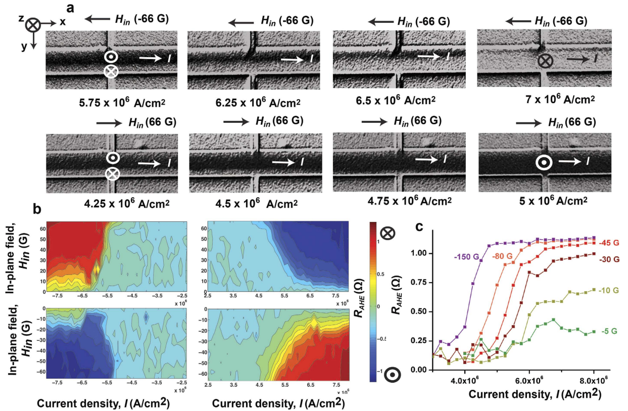
Figure 3. Movement of longitudinal domain wall orthogonal to the current. a, MOKE images of the magnetic bar after a positive current pulse of different magnitude is applied on a longitudinal domain wall (“mixed” state of Fig. 2a) in the presence of an in-plane field ( H_{in} ) in -x and +x direction. b, Contour plots of final R_{AHE} after application of a current pulse versus the magnitude of the current and magnitude of the applied in-plane field for different combinations of positive and negative currents and fields. c, Plots of R_{AHE} versus magnitude of current pulse for different values of magnetic field, applied in -x direction.
