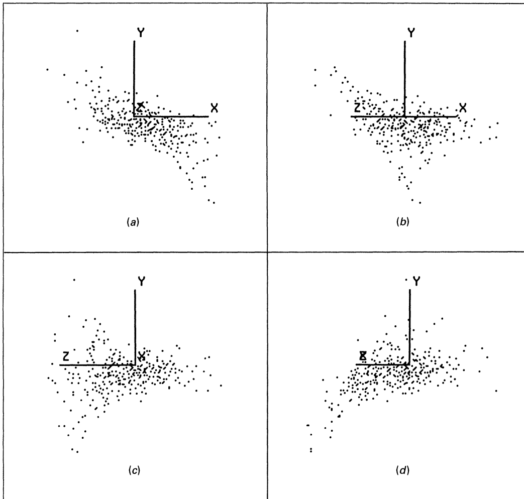
Figure 2. Best View of Data Generated From (6.3) With \sigma = .5 , \rho = 10 .
