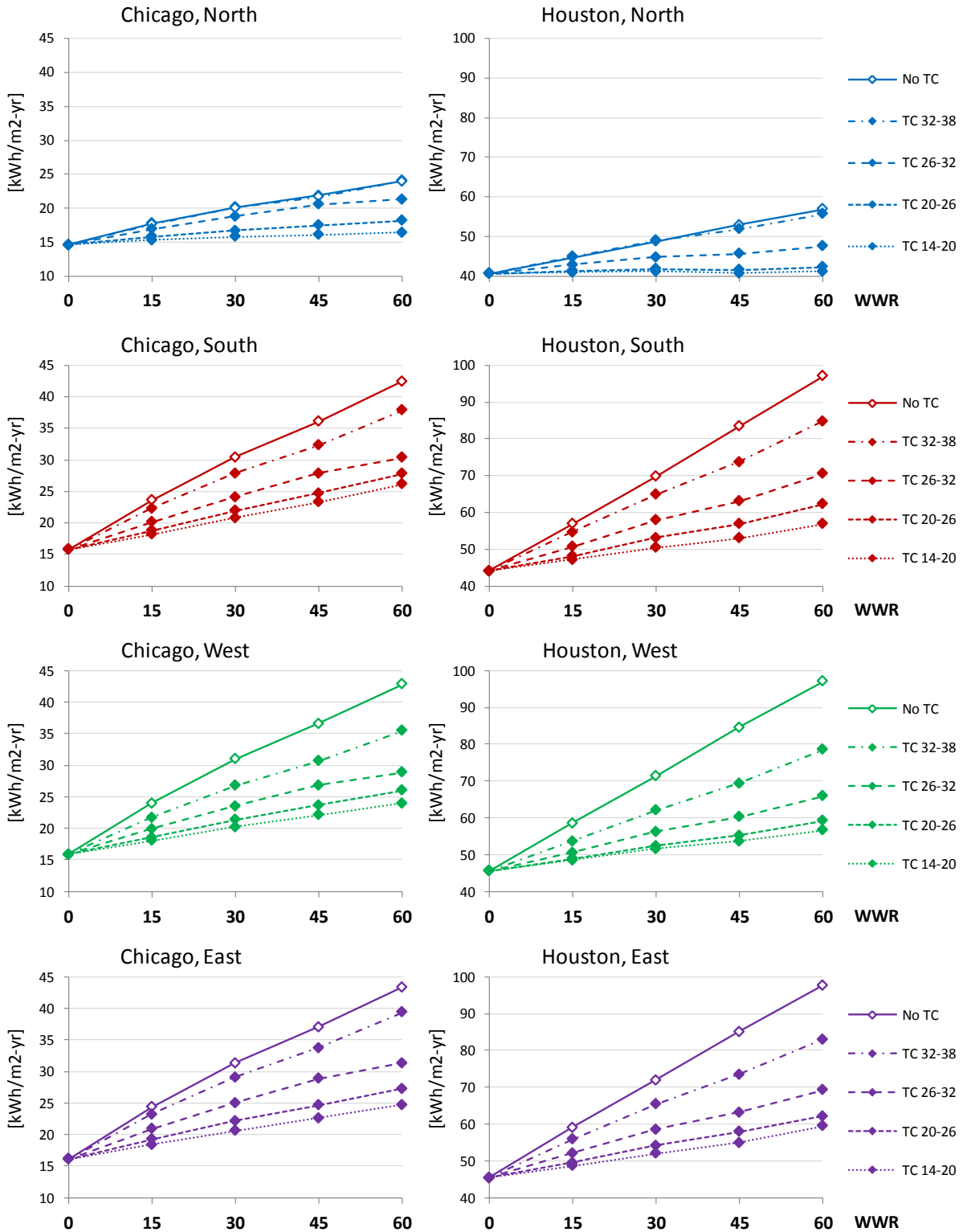
Annual site cooling energy use intensity (kWh/m 2 -floor-yr) for the reference window "No TC" and four thermochromic windows as a function of window-to-wall-area (WWR) ratio for four window orientations and the Chicago and Houston climates.
