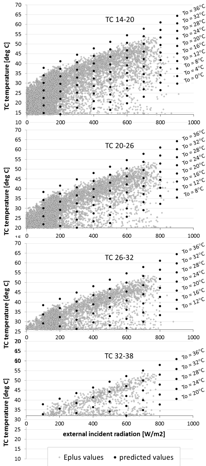
Fig. 6. Thermochromic glazing layer temperature ( ^{\circ}\text{C} ) versus incident radiation for hours when the thermochromic was in a partial or fully tinted state. Predicted TC glazing temperature values from linear regression (Equ. 1) are shown separately. EnergyPlus data are given for the four hypothetical thermochromic windows for the Chicago climate. All window orientations.
