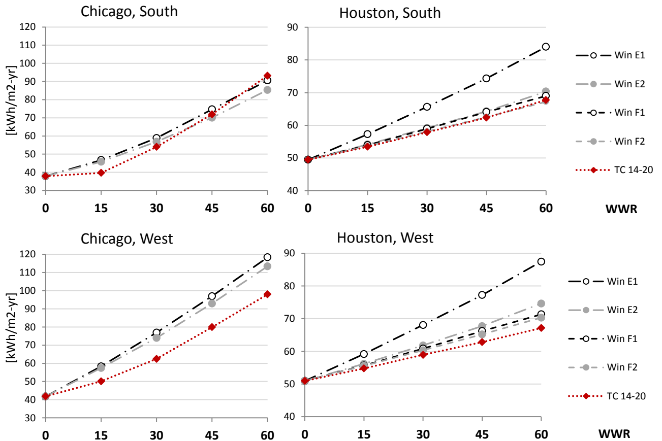
Fig. 13. Annual site energy use intensity ( \text{kWh/m}^2\text{-floor-yr} ) for heating, cooling, and ventilation for the hypothetical thermochromic window with a critical switching temperature range of 14\text{-}20^{\circ}\text{C} (TC 14-20), the near-IR low-e window without (E1) and with (E2) an indoor gray roller shade, and a highly-insulating window without (F1) and with (F2) and indoor shade. EnergyPlus data are given as a function of window-to-wall-area (WWR) ratio for south and west facing perimeter zones in the Chicago and Houston climates.
