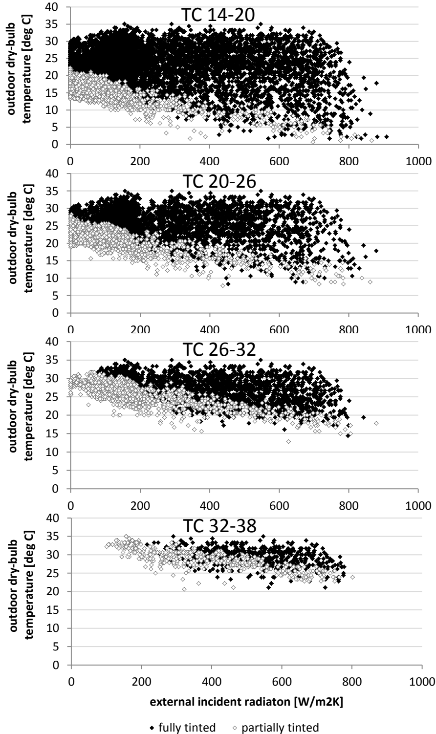
Fig. 5. Outdoor incident vertical irradiation ( \text{W}/\text{m}^2 ) and dry-bulb temperature ( ^{\circ}\text{C} ) that resulted in partial or full tinting of the four hypothetical thermochromic window types defined by different critical switching temperature ranges. The bold squares show the hours when the window was fully tinted, and the blank squares show the hours when the window was partially tinted out of a total of 35,040 hours (annual run for four orientations). Indoor air temperature was 21^{\circ}\text{C} . Data were produced by EnergyPlus simulations for the Chicago climate. All window orientations.
