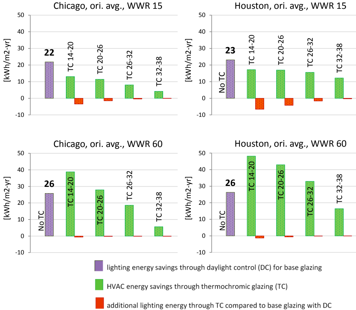
Fig. 14. Annual site lighting and HVAC energy use intensity savings ( \text{kWh/m}^2\text{-floor-yr} ) for the reference window “No TC” and four thermochromic windows with daylighting controls. Data for all orientations are averaged by zone floor area of the large office prototype (N/S:W/E = 4:3). Purple: Lighting energy savings of the “No TC” window with daylighting controls compared to the same window without controls. Red: Negative lighting energy savings of the four types of thermochromic windows compared to the “No TC” window. Green: Positive HVAC energy savings compared to the “No TC” window.
