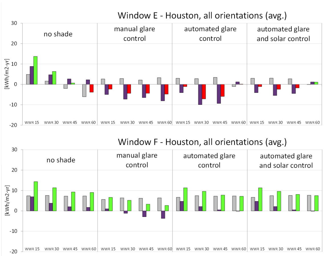
Fig. 16 B. Annual site lighting and HVAC perimeter zone energy use intensity savings ( \text{kWh/m}^2\text{-floor-yr} ) for the near-IR low-e window without (E1) and with (E2) an indoor gray roller shade, and a highly-insulating window without (F1) and with (F2) an indoor shade for different control algorithms compared to the TC 14-20 thermochromic window in Houston. All cases with daylighting controls. EnergyPlus data are given as a function of window-to-wall-area (WWR) ratio. Orientations are averaged by zone floor area of the large office prototype (N/S:W/E = 4:3). Gray: HVAC energy savings. Purple: Lighting energy savings. Red or Green: Net (less or more, respectively) annual energy savings compared to the TC 14-20 window.
