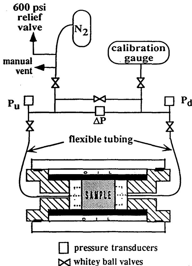
Figure 1. Gas-pressure-pulse-decay apparatus.
