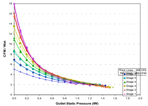
Carrier 58CVA090 furnace with prototype fan and GE ECM 4 Motor
