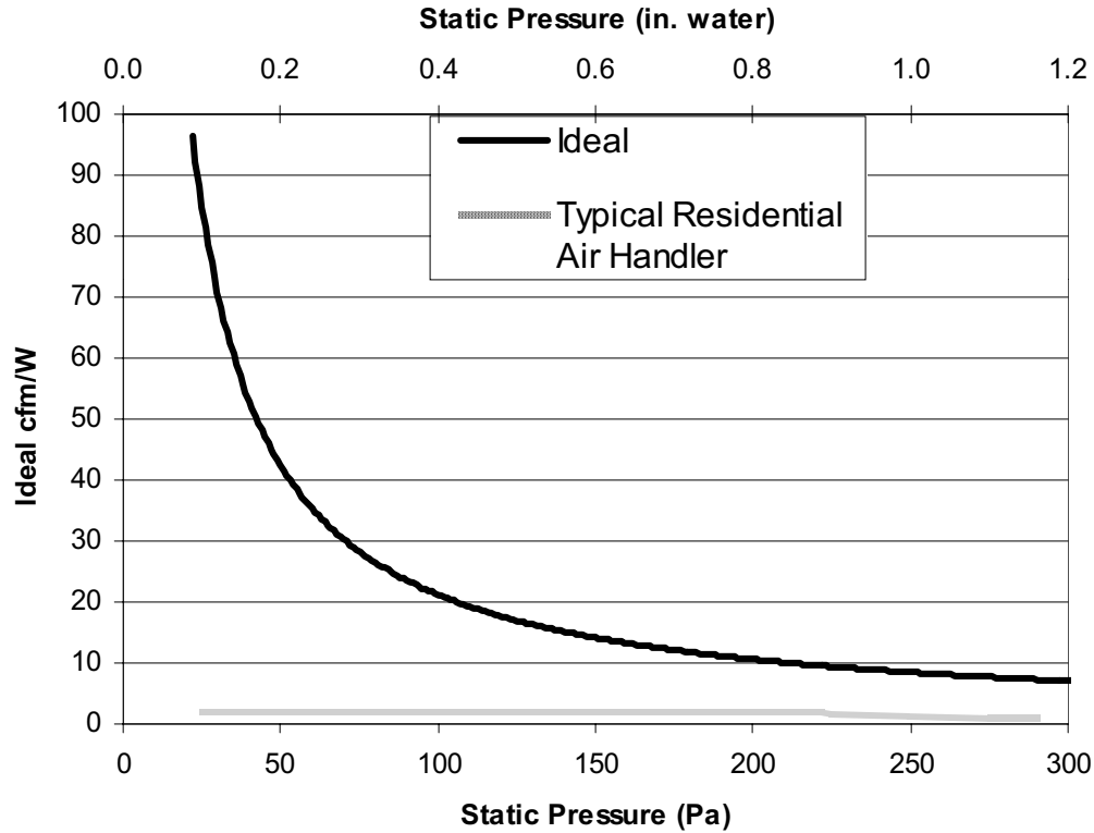
Figure 6. Maximum theoretical cfm/W for different static pressures compared to a typical residential unit
