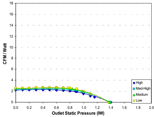
York P4HUA furnace with prototype fan and GE ECM 4 Motor
