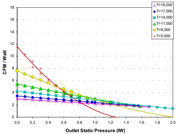
Carrier 58CVA090 furnace with prototype fan and GE ECM 4 Motor
