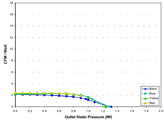
Carrier 58CVA090 furnace with standard fan and ECM 2 motor
