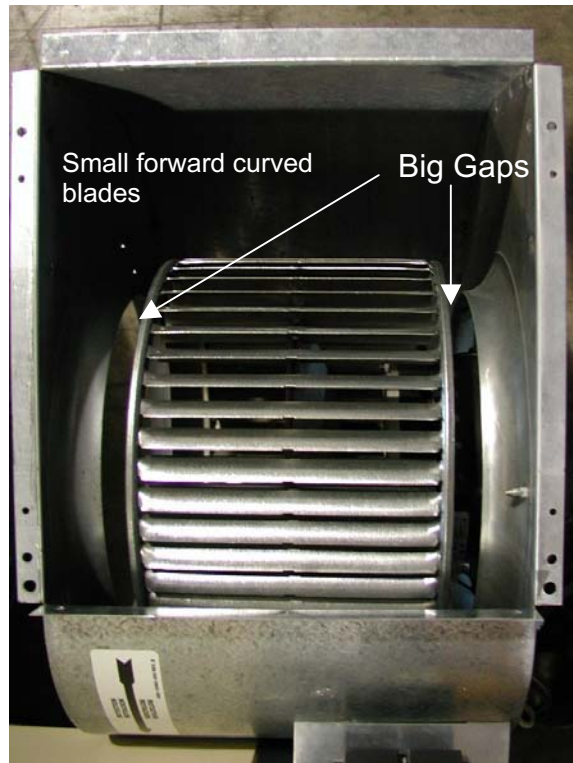
Figure 1. Typical air handler blower viewed from the air exit.
