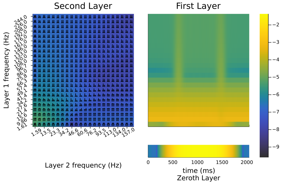
(a) ST Coefficients of the HeaviSine using Morlet wavelets of mean frequency \pi
