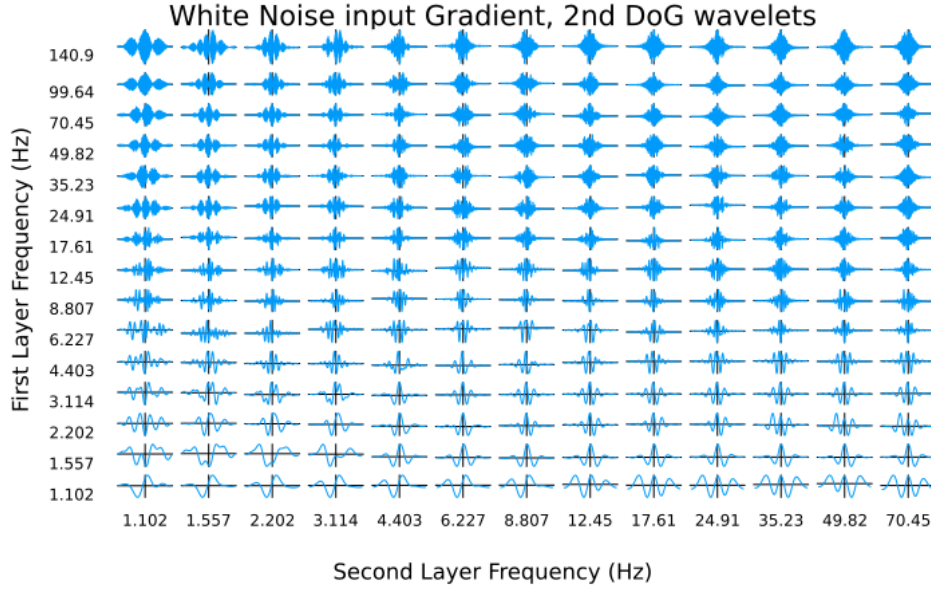
FIGURE 4.12. White noise, same format as Fig. 4.8
