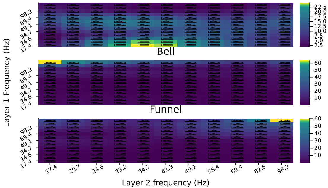
(a) Second layer transform of the fit coordinates, color is on a log scale
