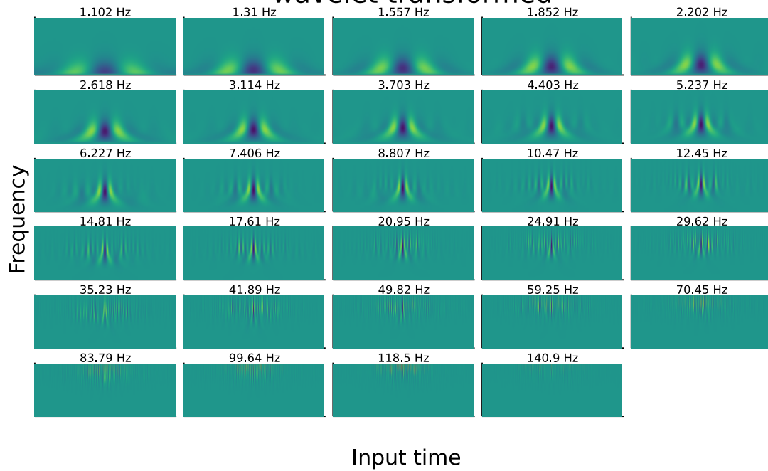
(a) Scalogram of the gradient of the first layer evaluated at the delta spike.
