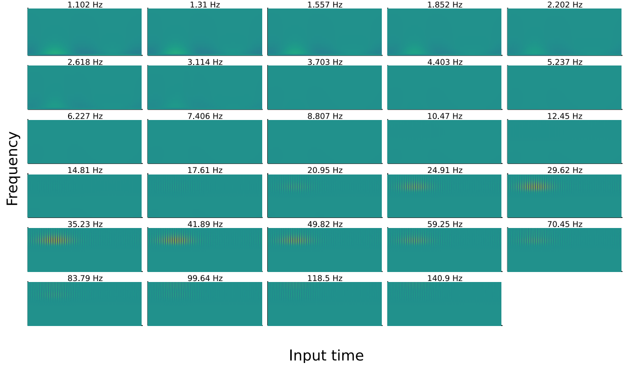
FIGURE 4.3. The scalogram using the first layer wavelets of the gradient \nabla_f s_{32}[\lambda] \Big|_{f=\sin} of a sinusoid of frequency 31.25Hz, centered at i/m = 32/128 .
