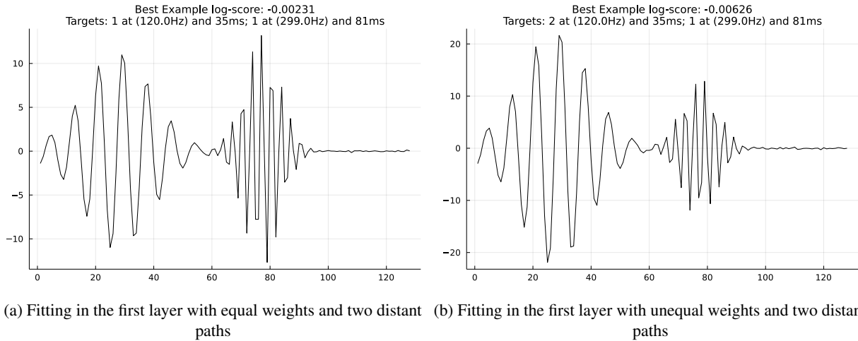
FIGURE A.7. Fitting multiple paths in the first layer
