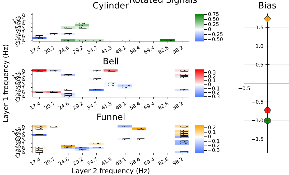
(b) Previously shown weights from Fig. 4.27 for ease of reference
