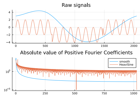
FIGURE 2.1. Comparing decay rates
