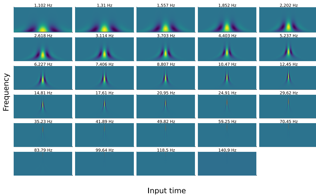
(b) Scalogram of the DoG2 wavelets for comparison.
