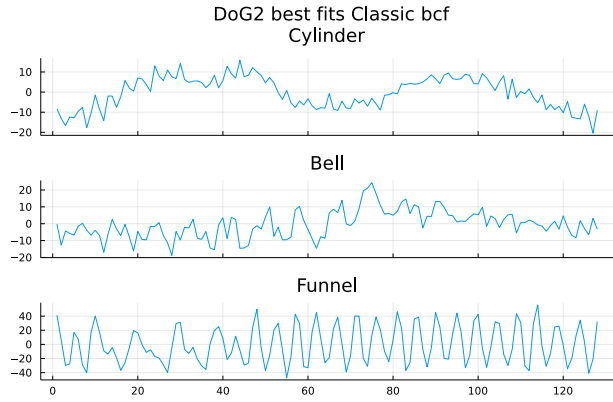
FIGURE 4.28. Pseudo-inverses of the lasso weight coefficients \beta^i for each class using only the second layer of a scattering transform using the 2nd DoG wavelets
