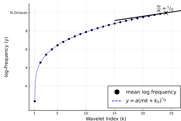
FIGURE 2.4. An example of the mean log-frequencies for some wavelets, where \beta = 4 and Q = 8
