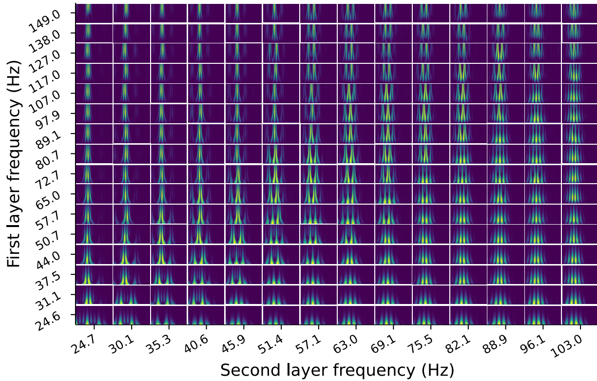
FIGURE 4.22. Scalograms for the DoG2 wavelets.
