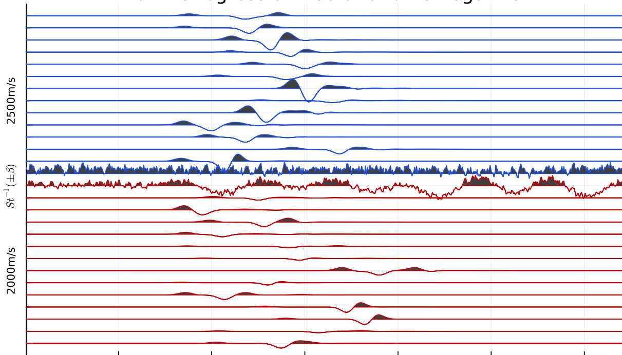
FIGURE 6.13. Comparing randomly selected signals from each speed with the pseudo-inverses emphasizing each respective speed. The first 13 blue signals are random examples at speed 2500m/s, while the last 13 red signals are random examples at speed 2000m/s. The first red signal is the pseudo-inverse of \beta in Fig. 6.11, which corresponds to maximizing the 2000m/s class, while the last blue signal is the pseudo-inverse for -\beta , which corresponds to maximizing the 2500m/s class.
