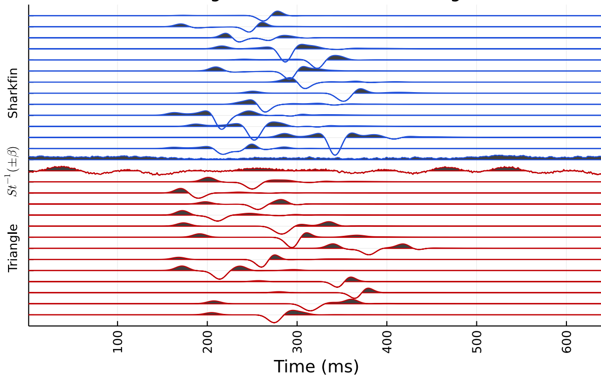
FIGURE 6.18. Comparing randomly selected signals from each shape with the pseudo-inverses emphasizing each respective shape. The first 13 blue signals are random sharkfin examples, while the last 13 red signals are random triangle examples. The first red signal is the pseudo-inverse of \beta in Fig. 6.16, which corresponds to maximizing the triangle class, while the last blue signal is the pseudo-inverse for -\beta , which corresponds to maximizing the sharkfin class.
