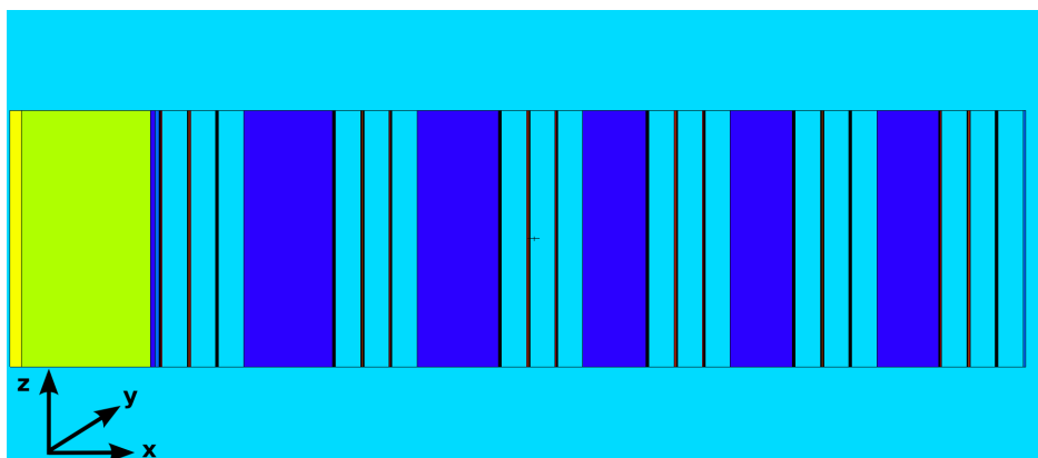
Figure 2.19: Simplified top-down MCNP6 model of the IPF Nb(p,x) target stack. The 100 MeV proton beam enters from the left of the figure, where it is incident upon the Inconel beam entrance window (yellow). The beam is transported down the length of the stack, towards the rear of the stack on the right side of the figure.
