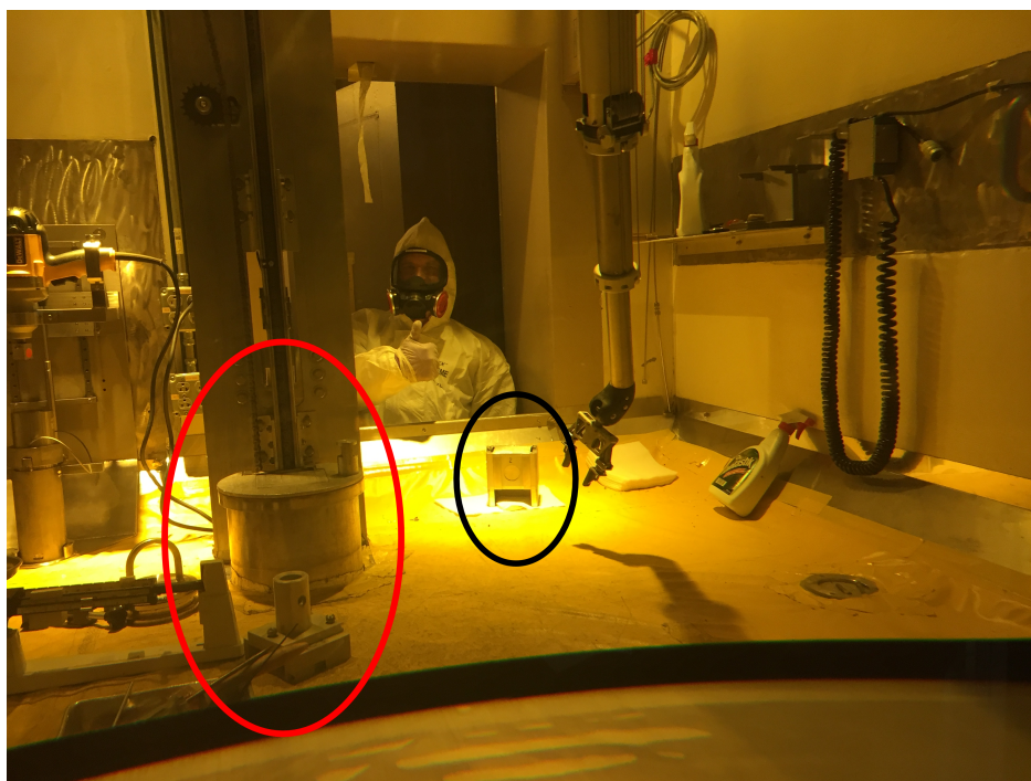
Figure 2.18: The IPF hot cell, used for lowering and retrieving the target stack (circled in black) and polyethylene beam profile monitors from the IPF beamline. Robotic manipulators are used for handling of all components in the hot cell, including mounting them onto a motorized track for insertion into the beamline. This track and mount are seen circled in red.
