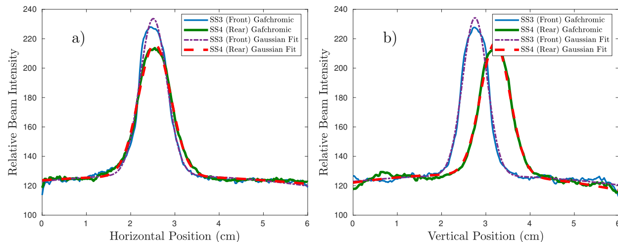
Figure 4.9: Relative beam intensity profiles for the radiochromic films seen in Figure 4.8. The intensity profiles were analyzed using ImageJ along (a) the major axis and (b) minor axis of each beam spot.
