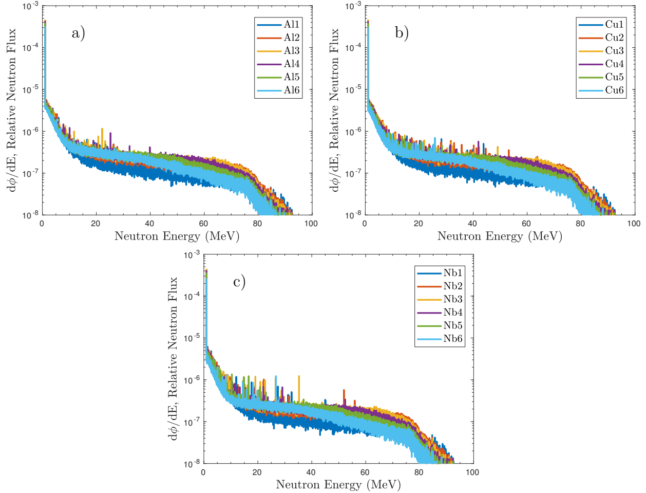
Figure 2.21: Final variance minimized incident neutron energy distributions for the (a) Al, (b) Cu, and (c) Nb foils, as simulated in MCNP6. The distribution tallies in each foil are all normalized to be per source proton, which was 10^8 in all simulations. As the beam is degraded, neutron energy distributions become visibly downscattered.
