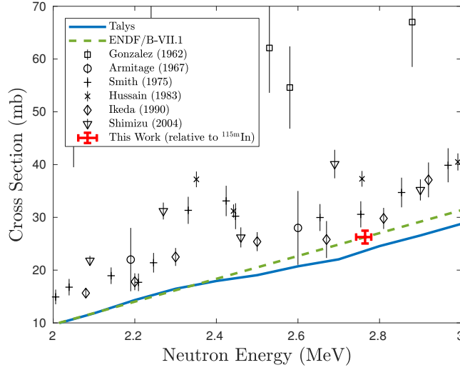
Figure 3.9: Measured ^{47}\text{Ti}(\text{n,p})^{47}\text{Sc} cross section relative to indium activation.
