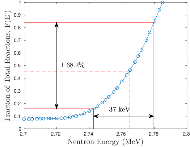
Figure 3.5: Fraction of total reactions induced in the Indium foil between the energies [0, E'] . The solid red boundaries indicate the energy region that corresponds to 68.2% of the total activation.
