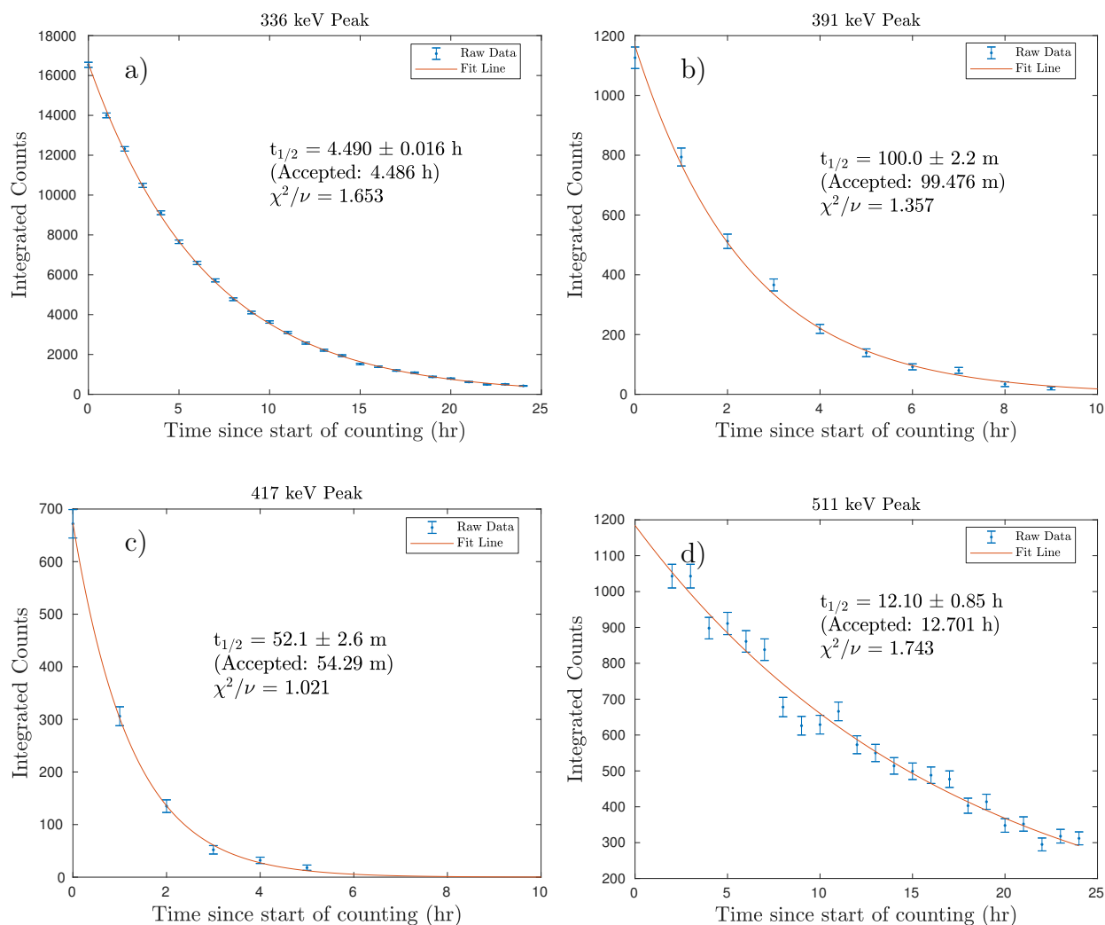
Figure 3.7: Decay curves used to verify photopeak transition assignment. (a) Decay curve for the isomeric transition of ^{115\text{m}}\text{In} [175], (b) decay curve for the isomeric transition of ^{113\text{m}}\text{In} [173], (c) decay curve for the \beta^- decay of ^{116}\text{In} [176], and (d) decay curve for the \beta^+ decay of ^{64}\text{Cu} [105].
