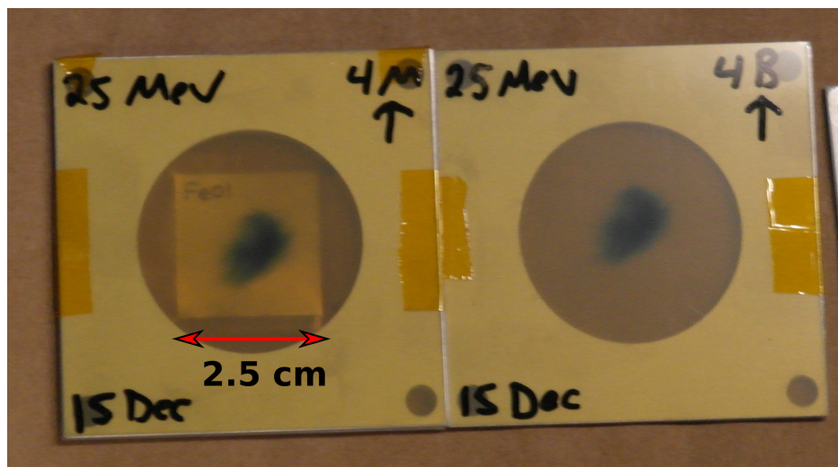
Figure 4.6: Final beam spot profile for the 25 MeV LBNL Fe(p.x) measurement. The proton beam is confirmed to be centered on the target position, and is focused to underfill the 25×25 mm target foils.
