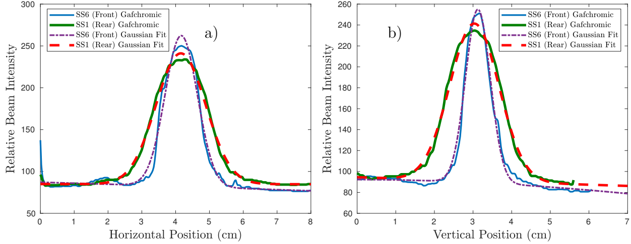
Figure 2.16: Relative beam intensity profiles for the radiochromic films seen in Figure 2.15. The intensity profiles were analyzed using ImageJ along (a) the major axis and (b) minor axis of each beam spot.
