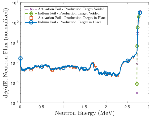
Figure 3.4: MCNP6-modeled neutron energy spectrum for the HFNG. The solid lines show the spectrum at the location of the indium and the activation foil. The dotted and dashed lines show the same with the neutron production target itself “voided” to remove scattering contributions.
