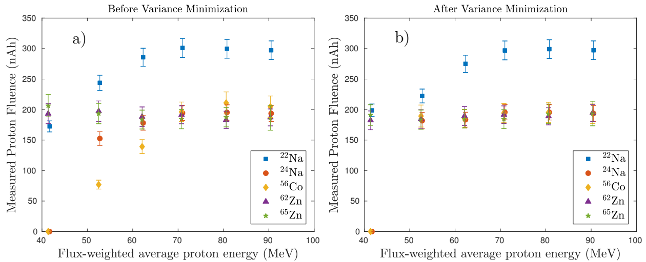
Figure 2.4: Results of variance minimization through enhancement of the effective areal density of the 6061 aluminum degraders by 2.52%. A noticeable reduction of variance in measured proton fluence is seen, particularly at the rear stack positions. Following minimization, additional apparent fluence is observed in the ^{\text{nat}}\text{Al}(\text{p},\text{x})^{22}\text{Na} and ^{\text{nat}}\text{Al}(\text{p},\text{x})^{24}\text{Na} monitor channels, due to contamination from ^{\text{nat}}\text{Si}(\text{p},\text{x})^{22,24}\text{Na} on the silicone adhesive used for sealing foil packets.
