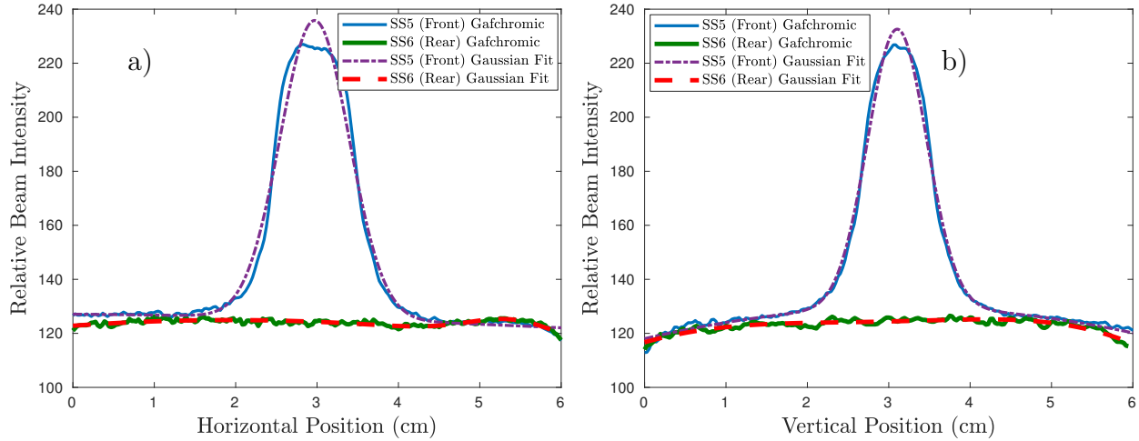
Figure 4.11: Relative beam intensity profiles for the radiochromic films seen in Figure 4.10. The intensity profiles were analyzed using ImageJ along (a) the major axis and (b) minor axis of each beam spot.
