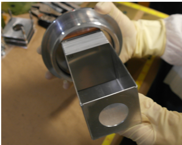
Figure 4.1: Photograph of the assembled 25 MeV target stack, before it was mounted in the beamline. The proton beam enters through the circular entrance in the foreground, and the upstream stainless steel profile monitor (SS-5) is visible at the front of the stack.
