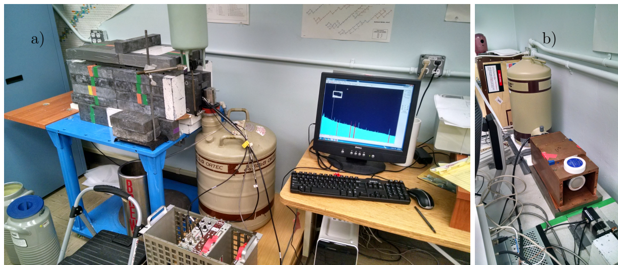
Figure 3.14: High-Purity Germanium Detectors used for gamma spectroscopy of the activated foils, as described in subsection 3.3.4. (a) Ortec 80% HPGe detector, (b) Ortec planar LEPS detector.
