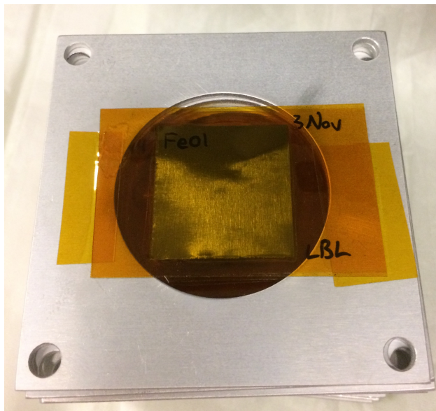
Figure 4.12: A stack of Fe, Cu, and Ti foils mounted on aluminum frames (Fe-01 visible on top), for the 55 MeV Fe(p,x) target stack. All foils are mounted over the aperture of a 1.5875 mm-thick aluminum frame.
