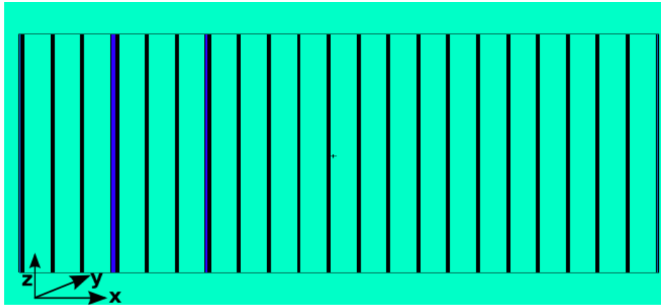
Figure 4.15: Simplified top-down MCNP6 model of the 25 MeV Fe(p,x) target stack. The proton beam enters from the left of the figure, where it is incident upon the SS-5 profile monitor. The beam is transported down the length of the stack, towards the rear of the stack on the right side of the figure.
