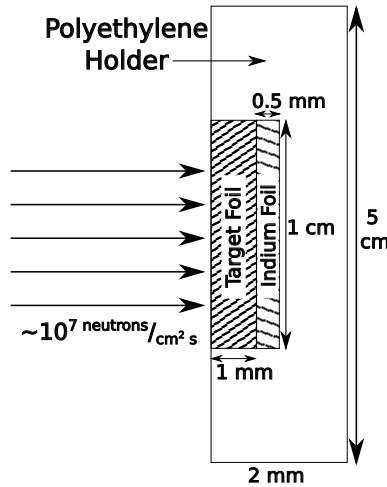
Figure 3.2: Schematic (not drawn to scale) of the sample holder used for the Berkeley HFNG.
