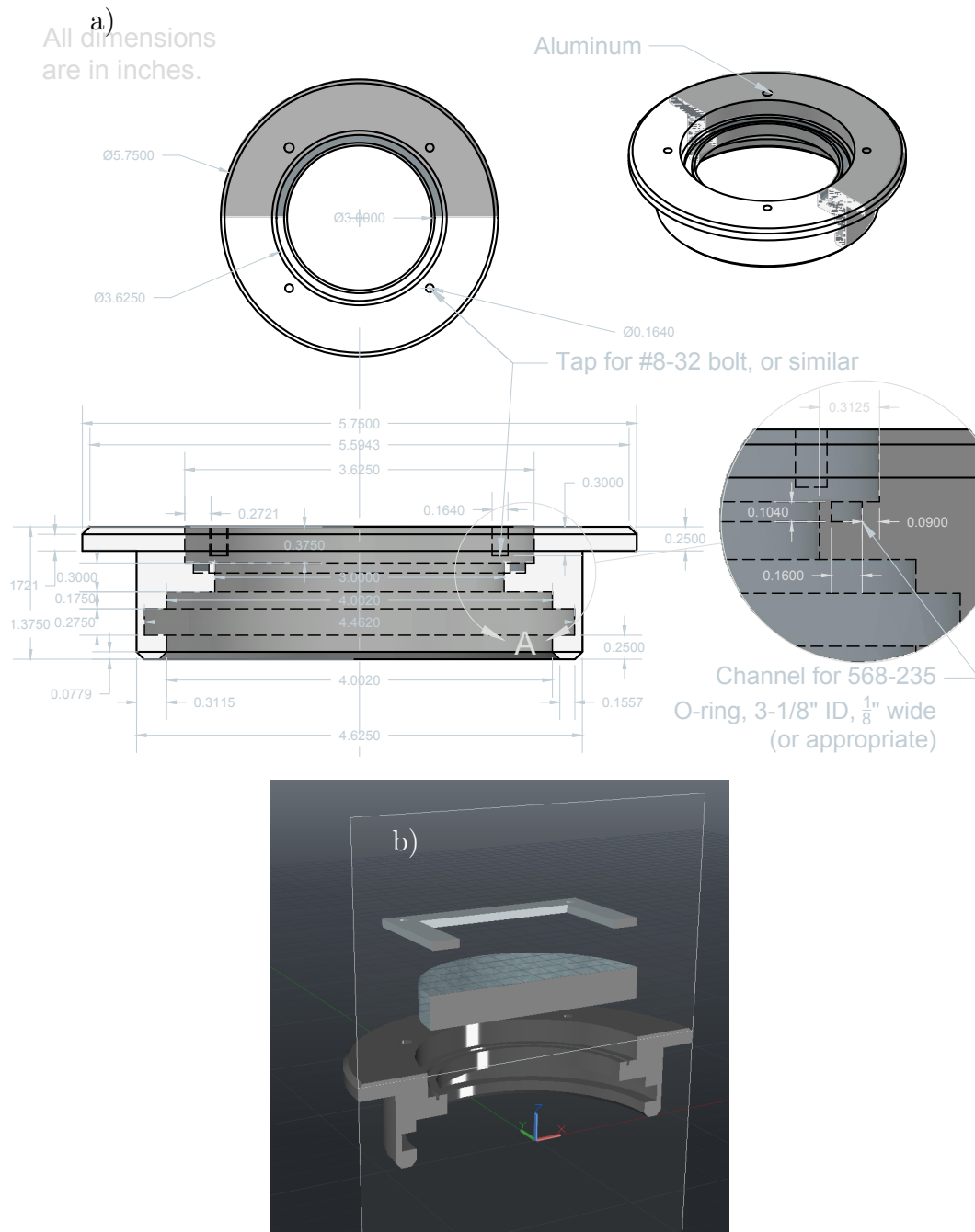
Figure 4.4: Blueprints (a) and 3D cutaway rendering (b) of the phosphor target used for real-time beam optics tuning at the 88-Inch Cyclotron.
