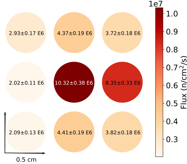
Figure 3.8: Relative fluxes as seen by a 3 x 3 array of indium foils. The central foil corresponds to the location in which target and monitor foils were mounted during the cross section measurements, verifying that the beam is centered on the middle of mounted foils.
