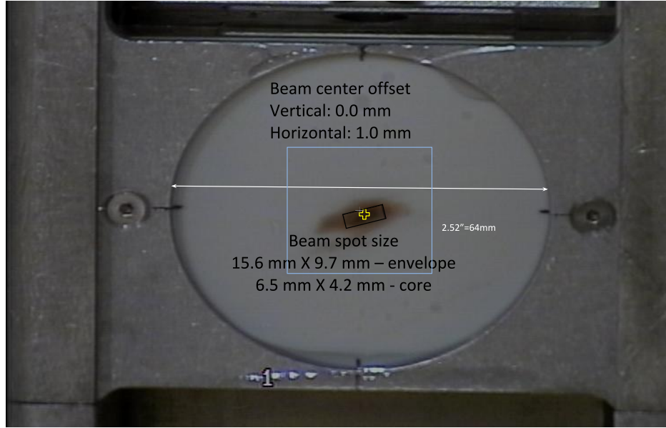
Figure 2.14: Final beam spot profile for the IPF Nb(p,x) measurement. The 100 MeV proton beam is confirmed to be centered on the target position, and is focused to underfill the 25×25 mm target foils.
