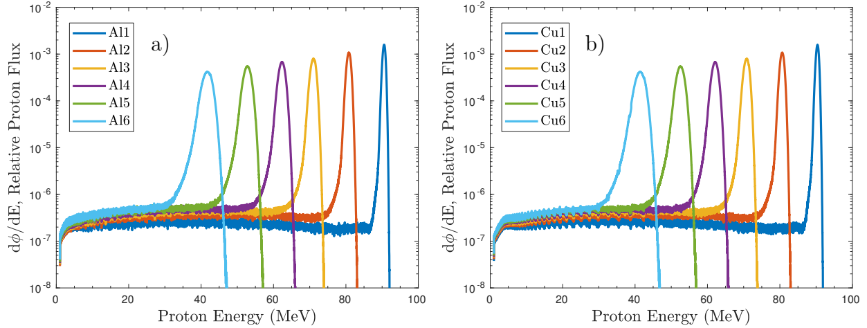
Figure 2.20: Final variance minimized incident proton energy distributions for the (a) Al and (b) Cu foils, as simulated in MCNP6. The distribution tallies in each foil are all normalized to be per source proton, which was 10^8 in all simulations. As the beam is degraded, proton energy distributions become visibly broadened due to straggling, and drop in magnitude due to scattering losses.
