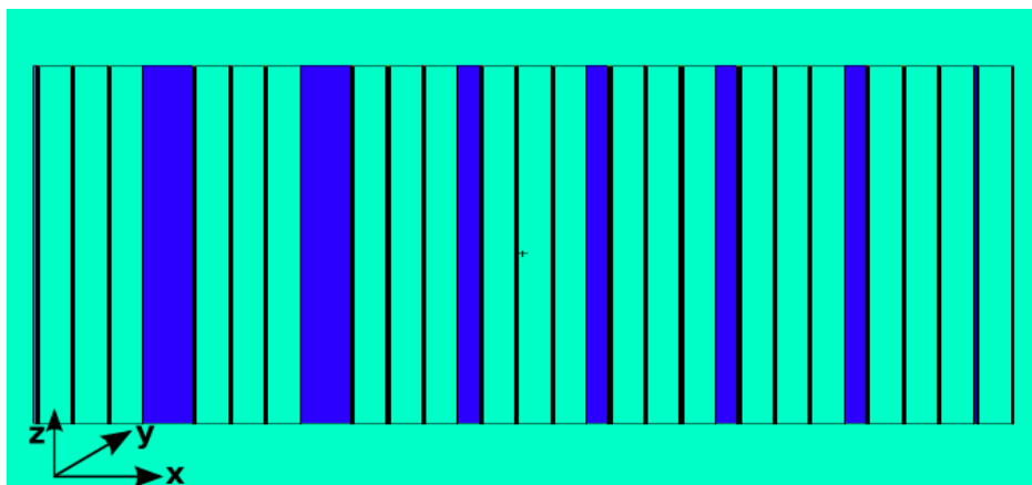
Figure 4.14: Simplified top-down MCNP6 model of the 55 MeV Fe(p,x) target stack. The proton beam enters from the left of the figure, where it is incident upon the SS-3 profile monitor. The beam is transported down the length of the stack, towards the rear of the stack on the right side of the figure.
