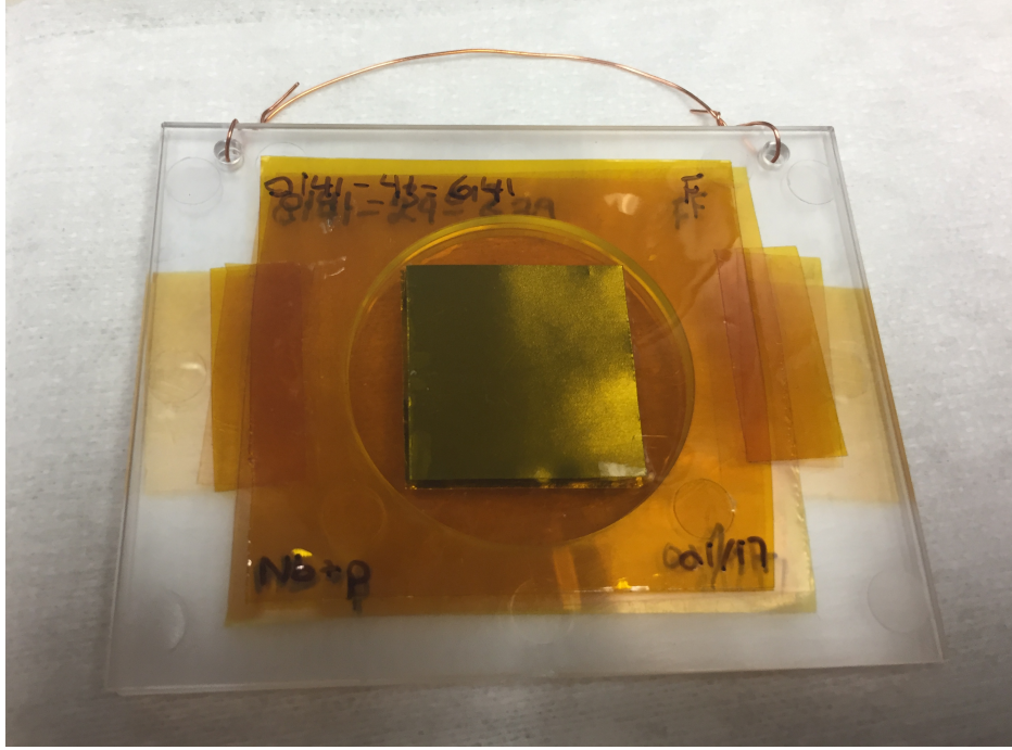
Figure 2.17: A stacked bundle of Nb (visible on top), Cu, and Al activation foils, for the 60 MeV position of the Nb(p,x) target stack. All foils are mounted over the aperture of a 1.575 mm-thick plastic frame and bundled together with baling wire.
