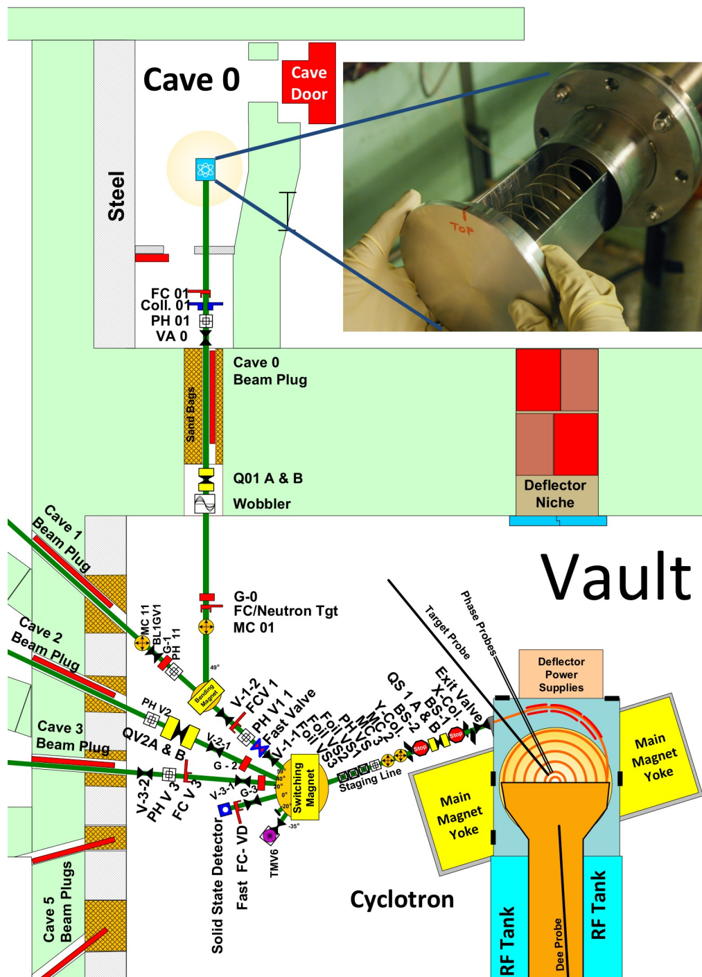
Figure 4.3: Schematic diagram of the 88-Inch Cyclotron facility and beamlines at LBNL, highlighting the beam path to Cave 0. A rear view of the target stack holder used in this work is seen here, where it mounts onto the end of the Cave 0 beamline.
