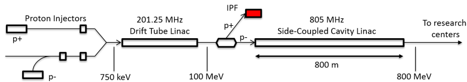
Figure 2.12: Schematic diagram of the LANSCE beamline at LANL. From the initial injectors, a proton beam is accelerated to 100 MeV in a drift-tube linear accelerator, where it is diverted away to the IPF beamline, highlighted in red.
