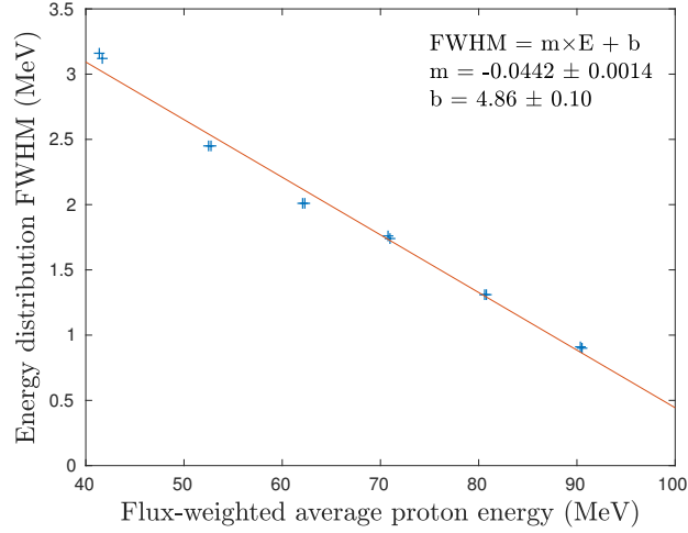
Figure 2.22: FWHM for the proton energy distributions of Cu and Al foils seen in Figure 2.20, as a function of the flux-weighted average proton energy.
