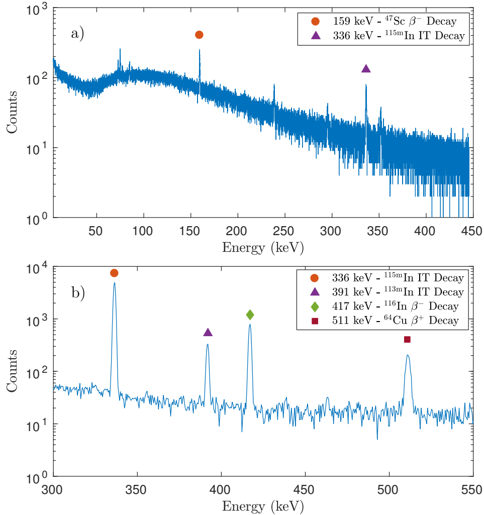
Figure 3.6: Example gamma spectra collected to monitor radioisotope production. (a) Gamma spectrum for the ^{47}\text{Ti}(\text{n,p})^{47}\text{Sc} production pathway foils, counted using a LEPS detector and (b) gamma spectrum for the ^{64}\text{Zn}(\text{n,p})^{64}\text{Cu} production pathway foils, counted using an 80% HPGe detector.
