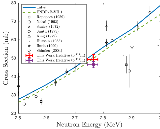
Figure 3.10: Measured ^{64}\text{Zn}(\text{n,p})^{64}\text{Cu} cross section relative to indium activation.
