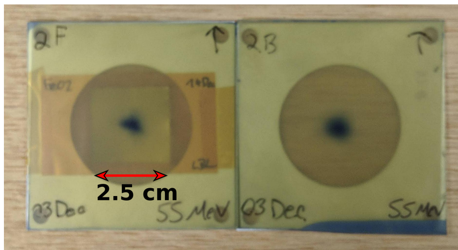
Figure 4.7: Final beam spot profile for the 55 MeV LBNL Fe(p.x) measurement. The proton beam is confirmed to be centered on the target position, and is focused to underfill the 25×25 mm target foils.
