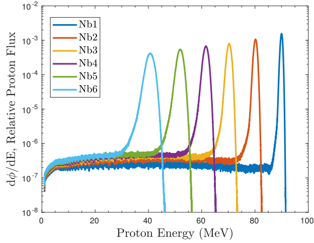
Figure 2.7: Final variance minimized incident proton energy distributions for the Nb foils, as simulated in MCNP6. The distribution tallies in each foil are all normalized to be per source proton, which was 10^8 in all simulations. As the beam is degraded, proton energy distributions become visibly broadened due to straggling, and drop in magnitude due to scattering losses.
