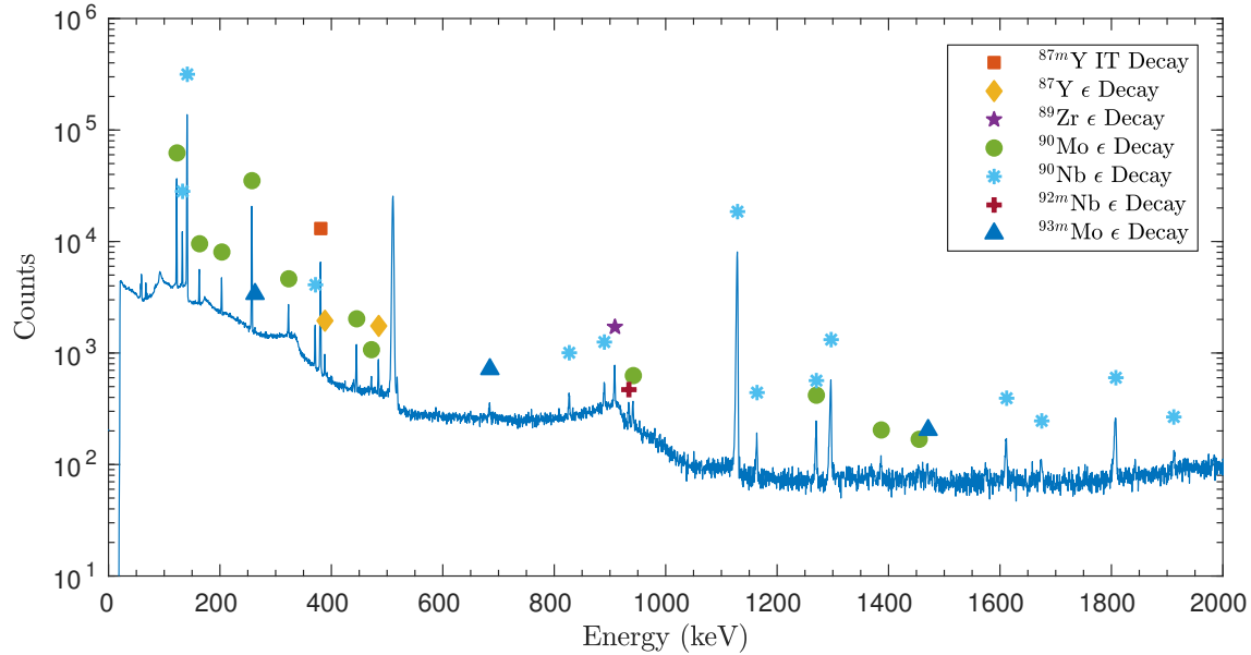
Figure 2.2: A gamma spectrum collected from an activated Nb foil at approximately 80 MeV. While the majority of observed reaction products are visible in this spectrum, the ^{90}\text{Mo} decay lines, which form the basis of the ^{93}\text{Nb}(p,x)^{90}\text{Mo} monitor reaction, are high in intensity and clearly isolated from surrounding peaks.
