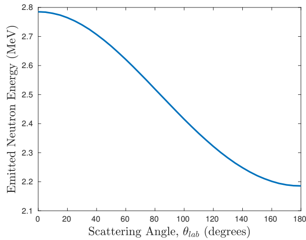
Figure 3.3: Energy-angle distribution for neutrons emitted following DD fusion, for 100 keV incident deuterons [169].
