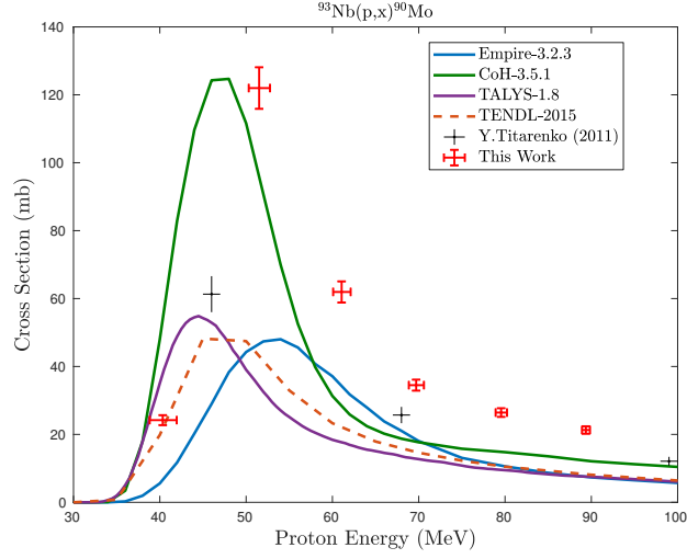
Figure 2.10: Measured ^{93}\text{Nb}(p,x)^{90}\text{Mo} cross section, with the ^{93}\text{Nb}(p,4n)^{90}\text{Mo} reaction channel visibly peaking at approximately 50 MeV.
