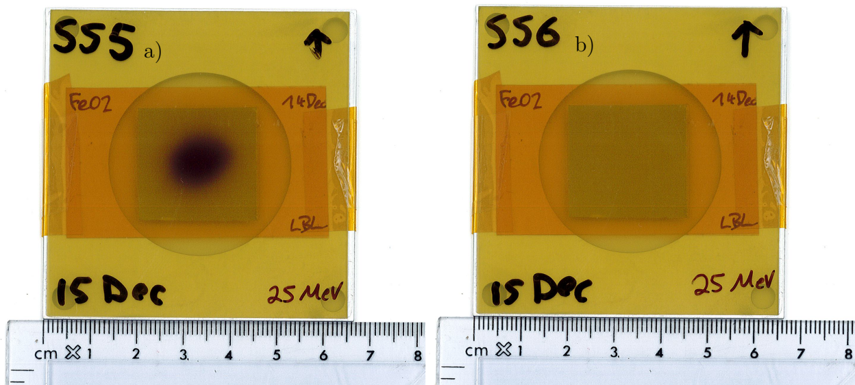
Figure 4.10: Radiochromic films for the 25 MeV LBNL Fe(p,x) measurement, developed by the stainless steel beam profile monitors in (a) the front of the stack (SS-5) and (b) the rear of the stack (SS-6). An unused iron foil is aligned behind each film, confirming that both the beam core and envelope underfilled the activation foils. No exposure is seen in the SS-6 film, as the beam was stopped upstream within the target stack, between Fe-14 and Ti-20.
