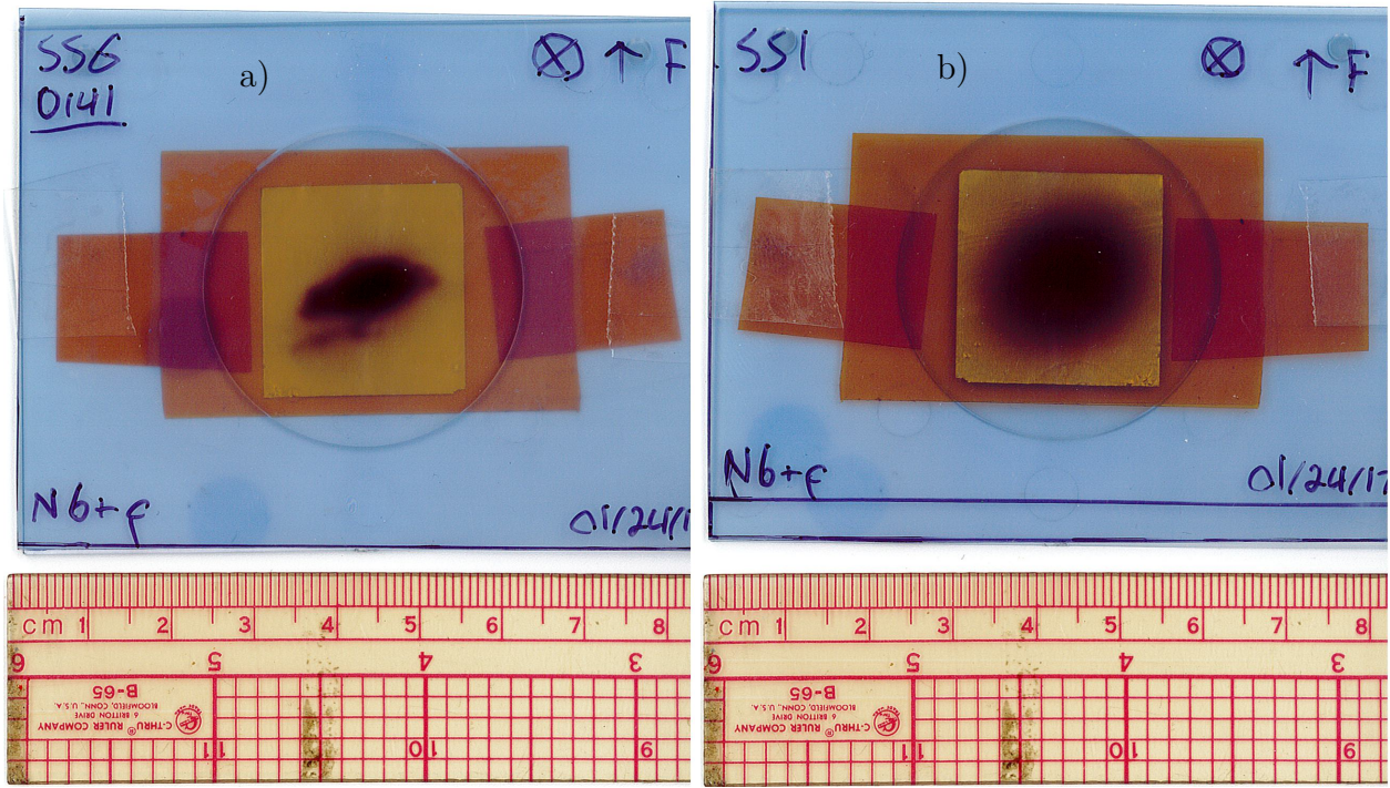
Figure 2.15: Radiochromic films for the IPF Nb(p,x) measurement, developed by the stainless steel beam profile monitors in (a) the front of the stack (SS-6) and (b) the rear of the stack (SS-1). An unused Al monitor foils is aligned behind each film, confirming that both the beam core and envelope underfilled the activation foils.
