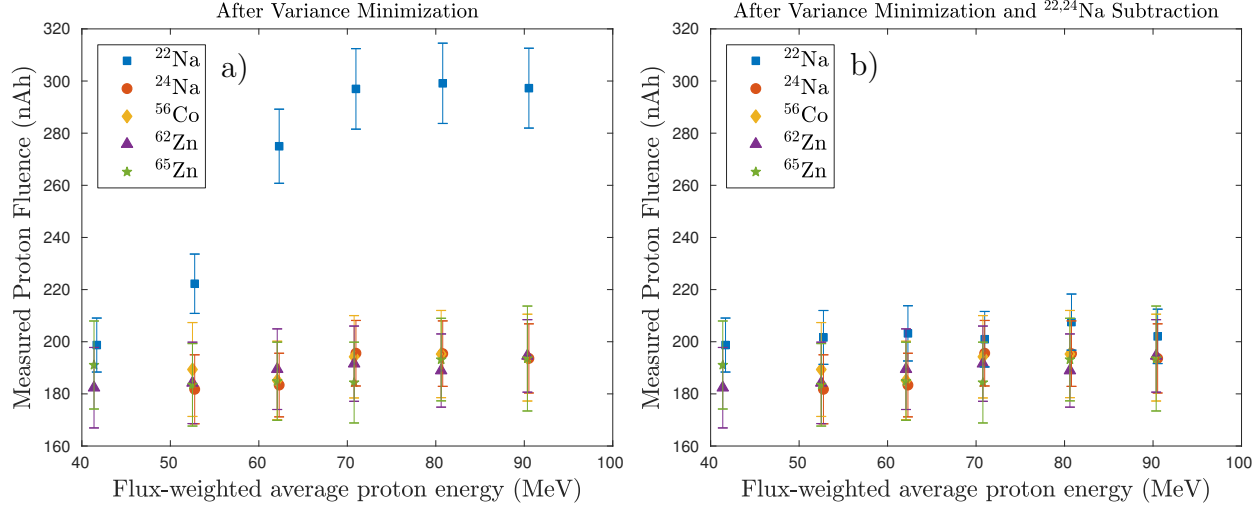
Figure 2.6: The “extra fluence” observed in the ^{\text{nat}}\text{Al}(p,x)^{22}\text{Na} and ^{\text{nat}}\text{Al}(p,x)^{24}\text{Na} monitor channels is caused by contamination from ^{\text{nat}}\text{Si}(p,x)^{22,24}\text{Na} on the silicone adhesive used for sealing foil packets. Following subtraction of ^{22,24}\text{Na} activities observed in the silicone adhesive of Nb and Cu foils in the same energy “compartment”, the consistency of the ^{\text{nat}}\text{Al}(p,x)^{22}\text{Na} monitor reaction improves dramatically. By excluding these contaminated channels, the remaining 3 independent monitor reactions serve to minimize uncertainty in stack energy assignments and incident fluence.
