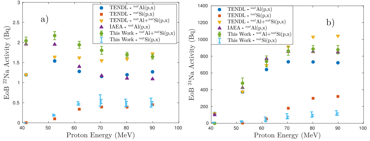
Figure 2.5: Estimates of EoB ^{\text{nat}}\text{Al}(p,x)^{22,24}\text{Na} and ^{\text{nat}}\text{Si}(p,x)^{22,24}\text{Na} activities using TENDL-2015 cross sections, in comparison with the IAEA recommended ^{\text{nat}}\text{Al}(p,x)^{22,24}\text{Na} cross sections. At low energies, experimentally observed apparent ^{22,24}\text{Na} activities in each Al foil packet are consistent with IAEA recommendations, but diverge at higher energies as the ^{\text{nat}}\text{Si}(p,x)^{22,24}\text{Na} exit channels begin to open up. ^{22,24}\text{Na} activities consistent with TENDL-2015 estimates are observed in each Nb and Cu foil packet as well, confirming that contamination may be attributed to activation of silicone adhesives.
