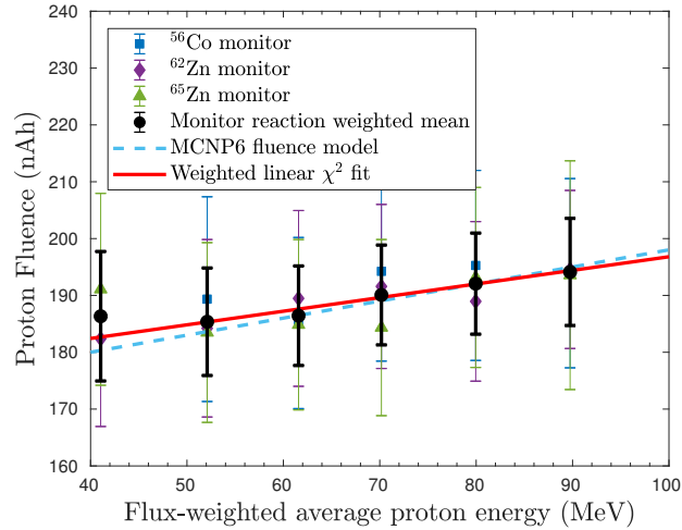
Figure 2.8: Final uncertainty-weighted mean proton fluences throughout the target stack, based on the variance-minimized observed fluence from the the ^{\text{nat}}\text{Cu}(\text{p},\text{x})^{56}\text{Co} , ^{\text{nat}}\text{Cu}(\text{p},\text{x})^{62}\text{Zn} , and ^{\text{nat}}\text{Cu}(\text{p},\text{x})^{65}\text{Zn} monitor reactions. The fluence drops by approximately 7.2–8.9% from the incident fluence of 196.9–198.8 nAh over the length of the target stack, based on fluence loss models from MCNP6 simulations and an empirical fit to fluence measurements.
