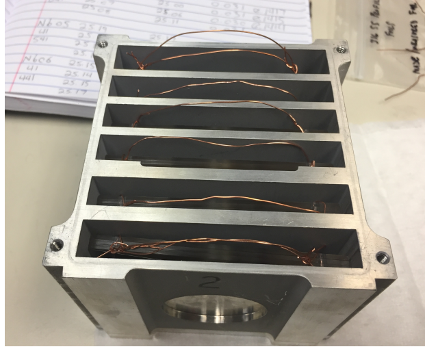
Figure 2.1: Photograph of the assembled IPF target stack, before the stack's o-ring lid was sealed in place. The baling wire handles affixed to each bunch of Al+Cu+Nb foils are visible in each energy position, to facilitate removal of activated foils via manipulators in the IPF hot cell. The circular Inconel beam entrance aperture is visible in the bottom center of the photograph.
