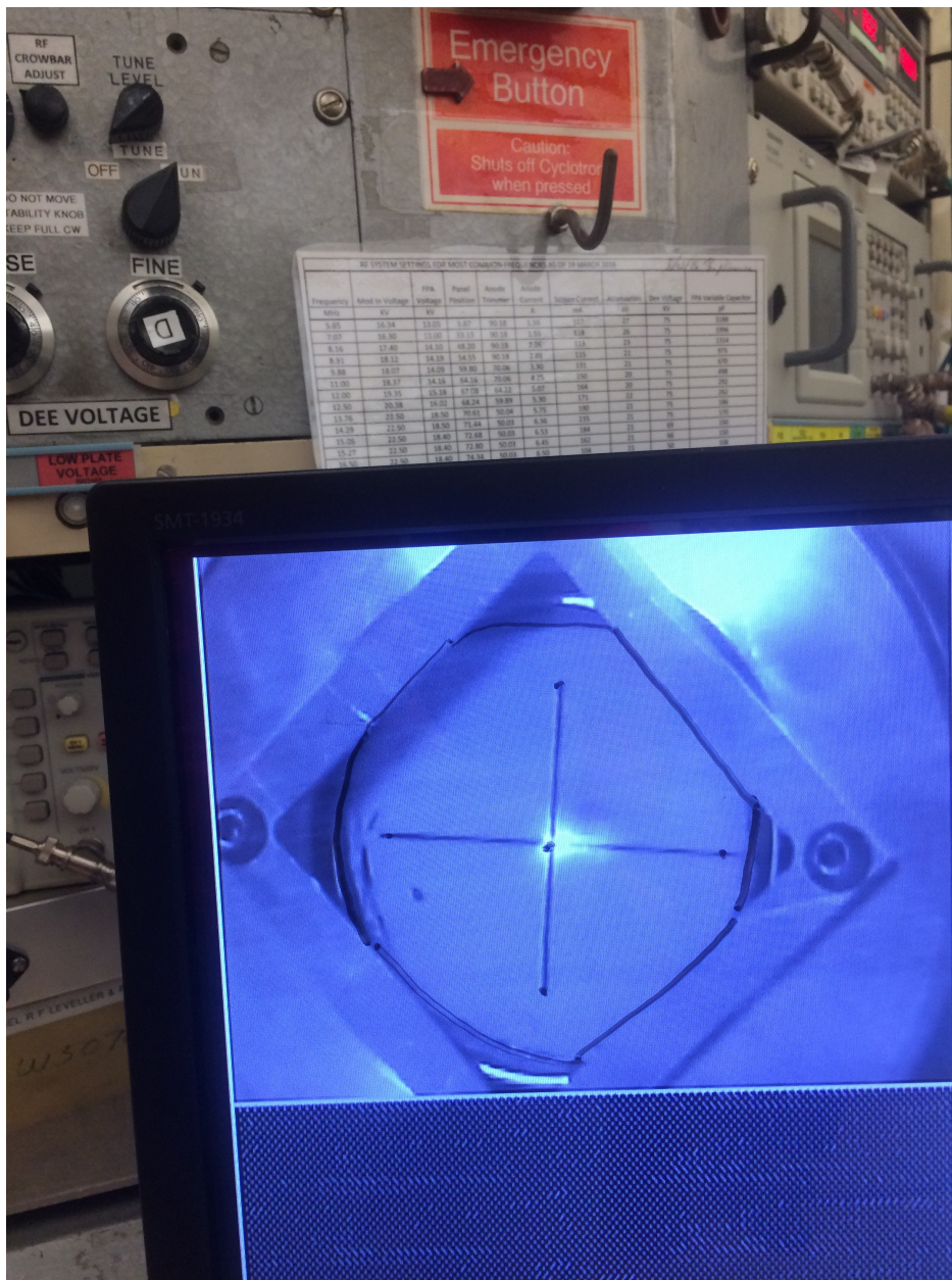
Figure 4.5: View of the remote feed of the phosphor target during beam optics tuning. The low-current proton beam used for tuning is visible as the bright glow around the reference crosshairs.
