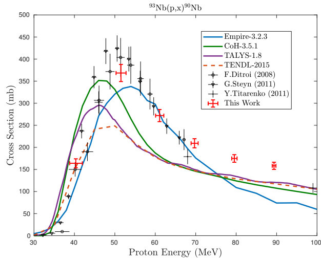
Figure 2.11: Measured ^{93}\text{Nb}(p,x)^{90}\text{Nb} cross section, with the ^{93}\text{Nb}(p,p3n)^{90}\text{Nb} reaction channel visibly peaking at approximately 50 MeV.
