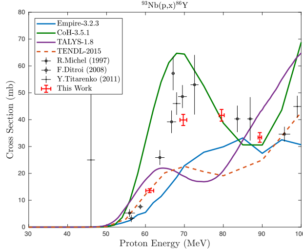
Figure 2.9: Measured ^{93}\text{Nb}(p,x)^{86}\text{Y} cross section, with the ^{93}\text{Nb}(p,\alpha p3n)^{86}\text{Y} reaction channel visibly peaking at approximately 70 MeV.
