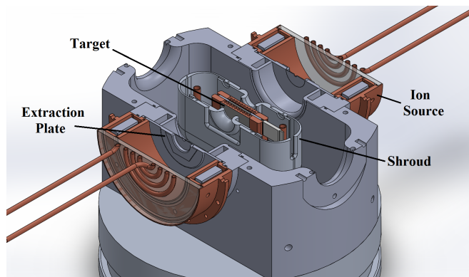
Figure 3.1: Cut-away schematic of the HFNG. The ion source is approximately 20 cm in diameter.
