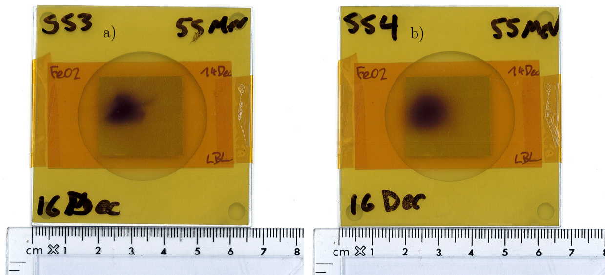
Figure 4.8: Radiochromic films for the 55 MeV LBNL Fe(p,x) measurement, developed by the stainless steel beam profile monitors in (a) the front of the stack (SS-3) and (b) the rear of the stack (SS-4). An unused iron foil is aligned behind each film, confirming that both the beam core and envelope underfilled the activation foils.
