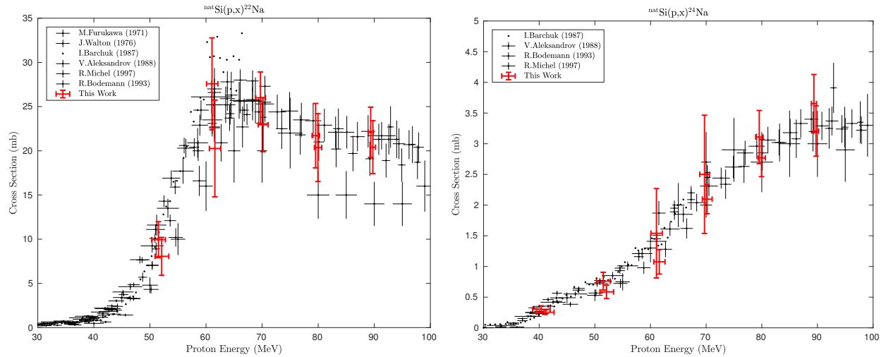
Figure 2.23: Apparent cumulative ^{\text{nat}}\text{Si}(p,x)^{22,24}\text{Na} cross section measurements, from production in the silicone adhesive of the Cu and Nb foils.
