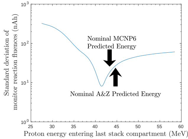
Figure 2.3: Result of the variance minimization performed by adjusting the degrader density in MCNP6 simulations of the target stack. A flux-weighted average proton energy of 41.34 MeV entering the last energy position creates a clear minimum in observed reaction fluence variance, corresponding to an areal density 2.52% greater than nominal. The variance minimum occurring at a lower incident energy than nominal MCNP6 and A&Z calculations indicates that there exists an additional systematic beam degradation not accounted for in modeling of proton transport in the stack design.
