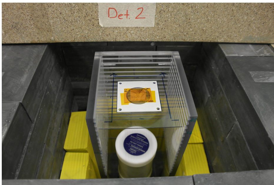
Figure 4.13: The ORTEC GMX Series (model #GMX-50220-S) High-Purity Germanium detector used for gamma spectroscopy of the activated foils, as described in subsection 4.2.2. The detector, counting foil Cu-14 in this figure, has a “ladder” permitting counting at various fixed distances (in 1 cm intervals) from the front face of the detector. With the lead shielding lid closed (for reduced background), the ladder permits counting up to 18 cm, and up to 75 cm with the lid open.
