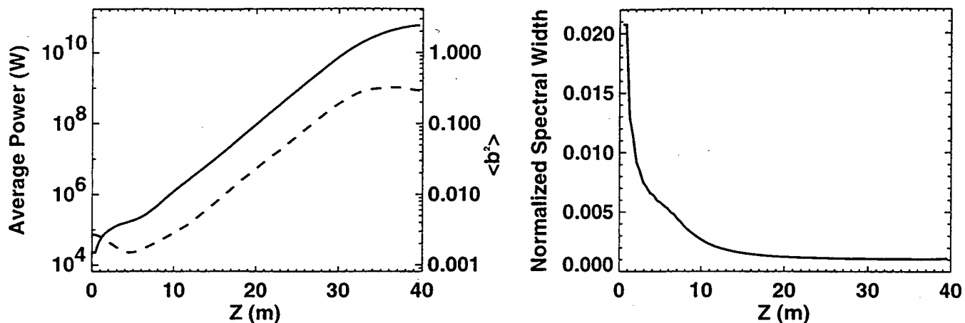
Figure 1. Results from a 2-D GINGER run starting from short noise using LCLS parameters of Table 1. The left plot shows the average radiation power (solid line) and the average electron beam bunching fraction squared as functions of undulator length z . The plot on the right shows the normalized RMS spectral width \Delta\lambda/\lambda_0 .
