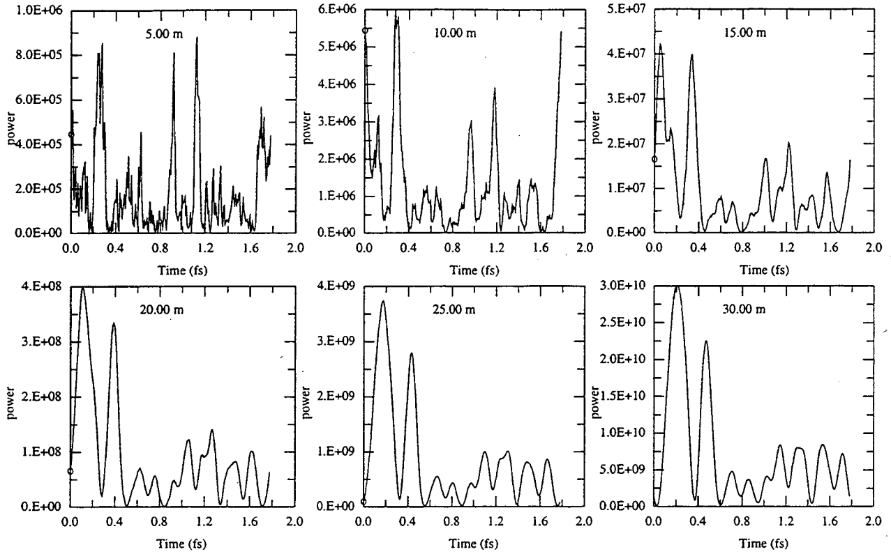
Figure 2. Snapshots of instantaneous power versus time at six z locations for the 2-D GINGER run of Fig. 1.
