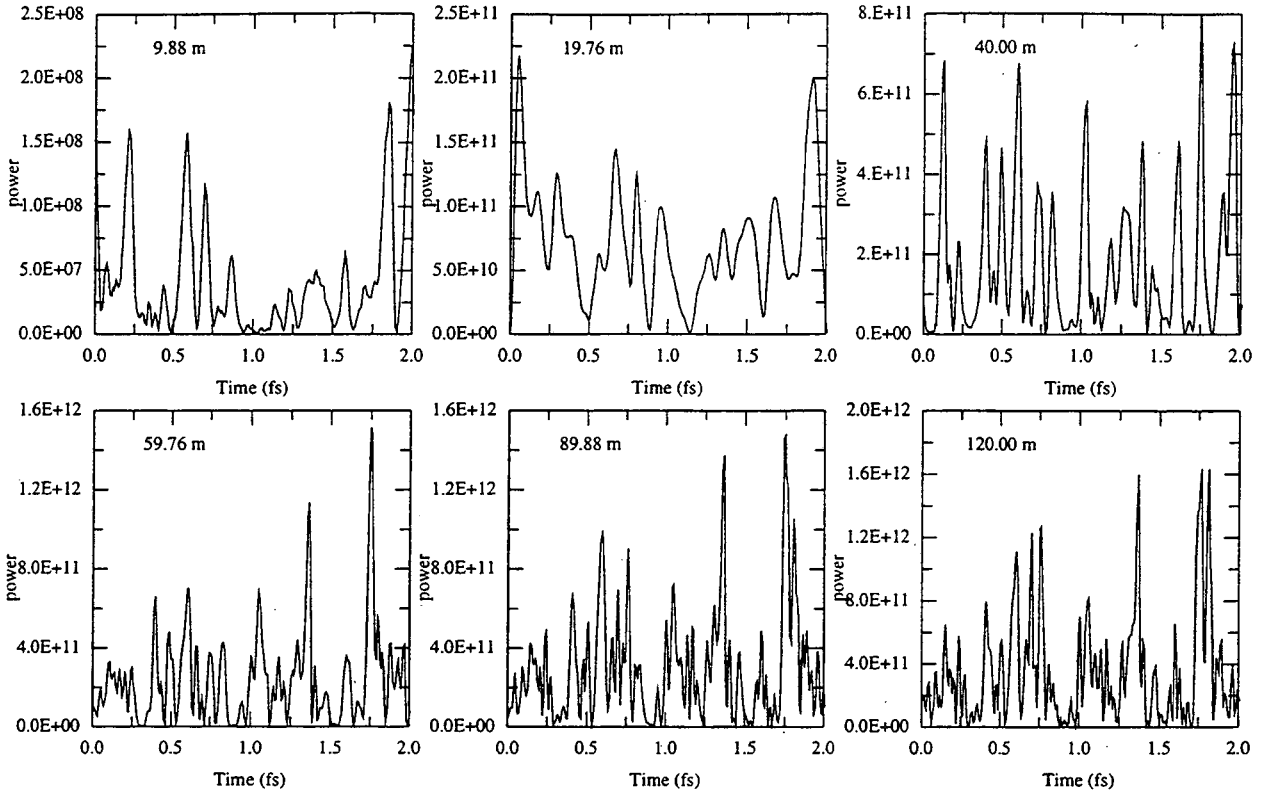
Figure 7. Snapshots of instantaneous power versus time at six z locations for a 1-D GINGER simulation starting from shot noise using the LCLS parameters described in Sec. 2.
