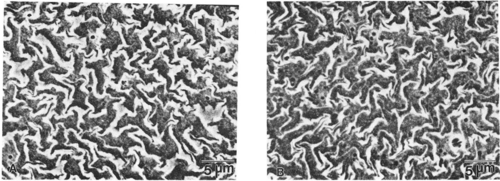
Fig. 5 SEM micrographs showing the cross section of the third stage at 1.032in (26.21 mm). The light regions are Nb and the dark are Nb-Ti, (a) 25vol% Nb and (b) 12.5vol%Nb.
