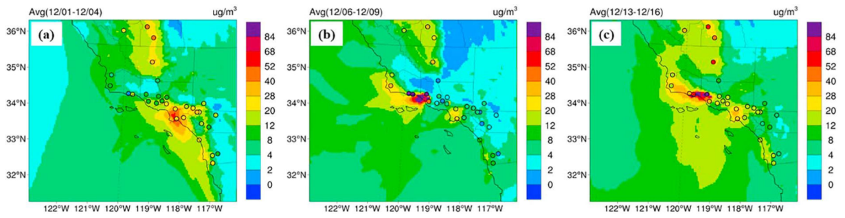
Figure 5. Overlay plots of the simulated (contour) and observed (circles) PM_{2.5} concentrations during the three stages: (a) the pre-Santa Ana wind stage, (b) the Santa Ana wind stage, and (c) the post-Santa-Ana wind stage.
