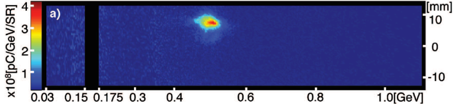
Figure 1: Single-shot electron beam spectrum from a 225 \mu\text{m} diameter H-discharge capillary with on-axis density 3.5 \times 10^{18} \text{ cm}^{-3} and a 1.5 J laser. The H-discharge capillary forms a plasma channel for guiding the laser. The 0.5 GeV electron beam contained 50 pc of charge, with 5.6% (rms) energy spread and 2 mrad (rms) divergence [10].
