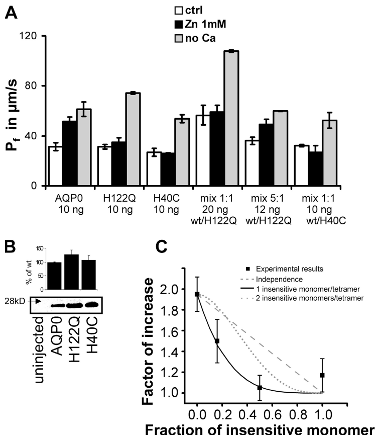
Figure 3. (A) Effect of 1 mM \text{ZnCl}_2 on the water permeability of coinjected AQP0 and a mutant insensitive to zinc H122Q or H40C. Mix 1:1 represents 10 ng of wild type and 10 ng of mutant H122Q (fraction of insensitive monomer = 10 divided by [10+10] = 0.5 ) and mix 5:1 represents 10 ng of wild type and 2 ng of mutant H122Q (fraction of insensitive monomer = 2 divided by [10+2] = 0.166 ). In both mixtures, the effect of zinc was dramatically diminished but the calcium sensitivity remained intact. Mix 1:1 represents 5 ng of wild type and 5 ng of mutant H40C. (B) Western Blot of uninjected oocyte membranes, AQP0, mutant H122Q, and mutant H40C. A band, lower than the 28 kD marker, was seen in AQP0, H122Q, and H40C and not seen in uninjected oocytes. The bar graphs represent the average of scanned bands from three different experiments. There was no noticeable difference between the wild type and the mutant expression level. (C) Theoretical curves predicting the factor of increase, assuming the monomers behave independently (gray dashed line) or one or two insensitive monomers can block zinc sensitivity (black continuous line and gray dotted line respectively). Experimental results are plotted as filled squares and are well fit by the one insensitive monomer curve. Each data point is the average of experiments using nine oocytes from three different batches.
