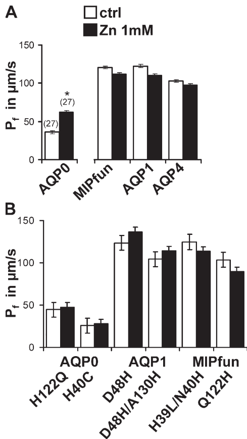
Figure 1. (A) Effect of 1 mM ZnCl 2 on the water permeability of AQP0, MIPfun, AQP1, and AQP4. Only AQP0 showed zinc-induced increase in water permeability (from 35.9 ± 2.5 to 62.3 ± 5.5 µm/s). (B) Effect of 1 mM ZnCl 2 on the water permeability of mutants of AQP0, AQP1, and MIPfun. They all lacked the zinc sensitivity. *, different from control at a significance of P < 10^{-5} using the Student's t distribution. Unless otherwise noted, each data point is the average of experiments using nine oocytes from three different batches.
