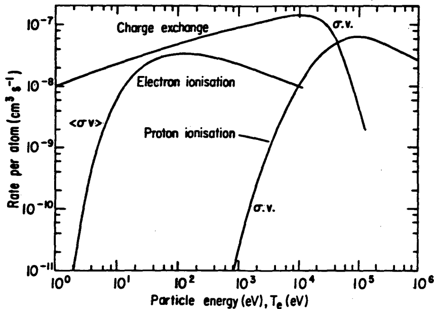
Fig. 2. Reaction rates for atomic hydrogen for electron impact ionization, proton impact ionization, and charge exchange with protons as a function of lab hydrogen energy. The energy scale for the electron ionization rate is the electron temperature.
