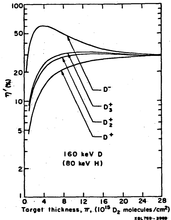
Fig. 22. The approach to equilibrium with increasing target thickness.
