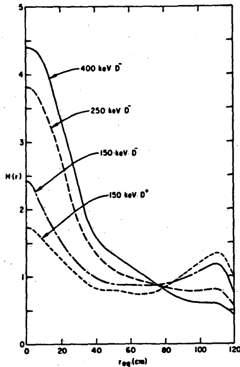
Fig. 3. Neutral beam deposition profiles for 150, 250, and 400 keV D^- based beams and for a 150 keV D^+ based beam on small version of the proposed FED tokamak. 13
