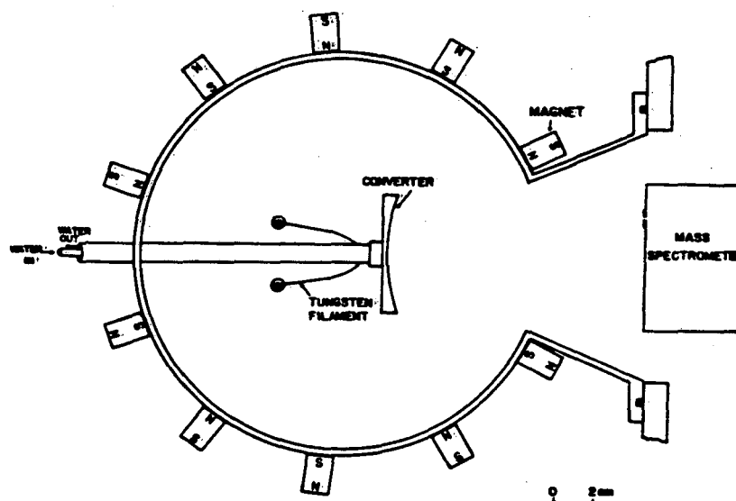
Fig. 25. Schematic of a surface-production negative ion source. The Mo "converter" is in a plasma containing hydrogen and cesium ions, and is biased positive with respect to the plasma.
