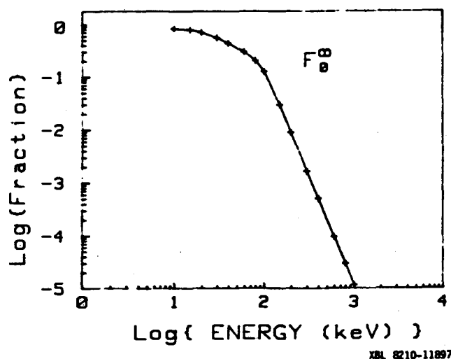
Fig. 21. The neutralization efficiency for a thick target \sigma_{10}/(\sigma_{10} + \sigma_{01}) .
