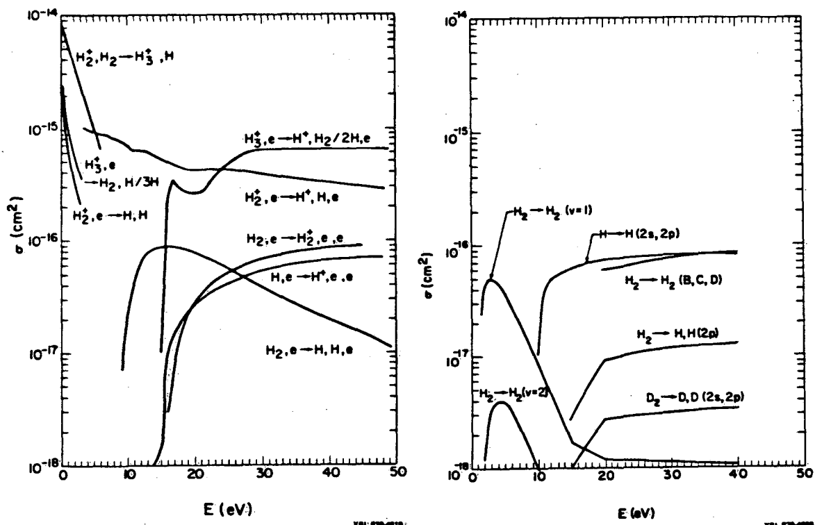
Fig. 17. Cross sections of reactions occurring in the volume of a hydrogen plasma.
