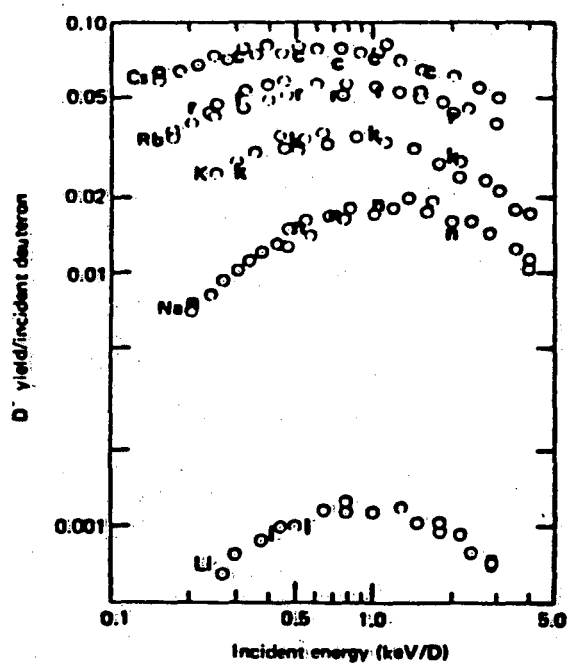
Fig. 24. Negative ion secondary emission coefficients for pure alkali metals.
