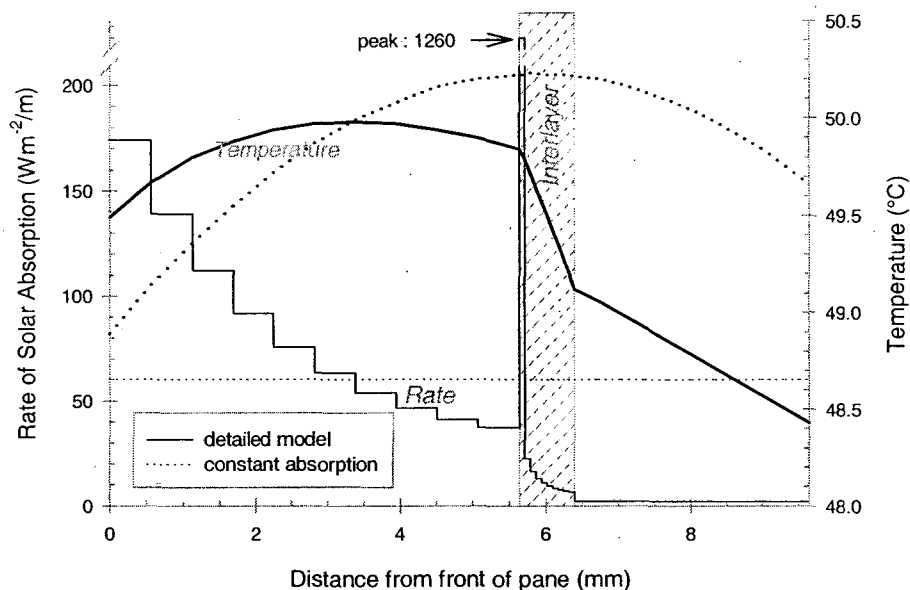
Figure 5. The local rate of solar absorption and temperature profile inside a laminate consisting of 6 mm tinted glass outboard lite with a reflective solar control coating on #2 surface, 0.76 mm clear PVB interlayer and 3 mm clear glass inboard lite. The position of the interlayer in the laminate is indicated by the shaded region..
