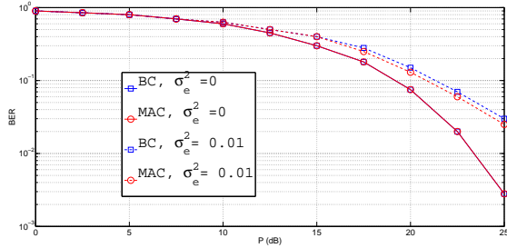
Fig. 4. BER versus P . K = 3 , M = 2 , N = 10 , P_L^M = P_1^B = 20\text{dB} .
