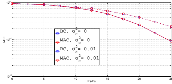
Fig. 3. MSE versus P . K = 3 , M = 2 , N = 10 , P_L^M = P_1^B = 20\text{dB} .
