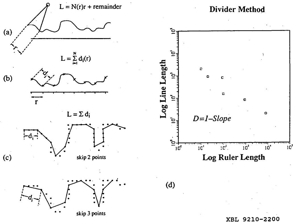
Figure 6. Divider (ruler) method: caliper or divider applied to surface of profile (a); modified divider where straight line length between divisions along base are measured (b); digitized ruler method using point counting (c) (Clark, 1986); example of plotted measurements where D = 1 - \text{slope} (d).
