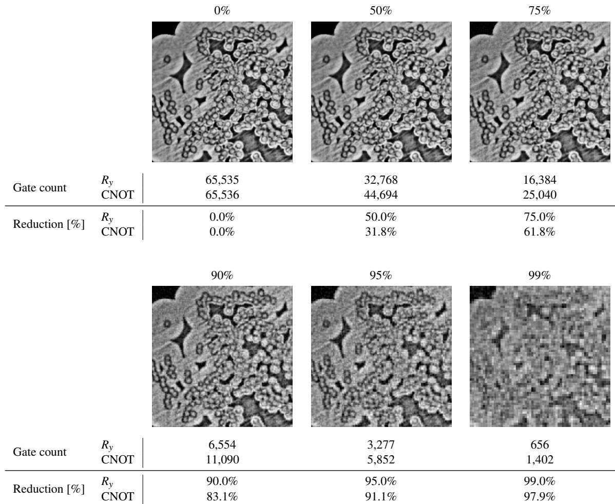
Figure 6. 256 \times 256 image data from of a ceramic matrix composite sample 49 acquired using microCT simulated with QPIXL++ at various compression levels and corresponding gate counts of the 17-qubit U_{\mathcal{R}} circuit. The final two rows list the reduction in R_y and CNOT gates compared to the uncompressed circuits.
