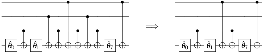
Figure 2 illustrates the compression algorithm for an actual image of 8 pixels where all transformed angles \hat{\theta}_i below the tolerance \delta = 0.01 are set to zero. Note that, although the compression can influence all the angles \theta_c , the changes of the grayscale values are only in the range of [-3, 3] . The reason for this is that Eq. (18) is well-conditioned so that small changes in \hat{\theta} only lead to small changes in \theta and its corresponding grayscale values.
