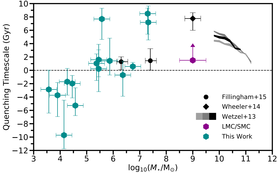
Figure 5.4: The quenching timescale as a function of satellite stellar mass for our primary sample of MW dwarfs (cyan hexagons). We include an estimate of the quenching timescale for both the SMC and LMC (magenta hexagon) based on a lookback time to first infall of 1.5 Gyr from Kallivayalil et al. (2013). The black data points and grey bands illustrate the results of statistical studies of satellites in groups and clusters (including the Local Group, Wetzel et al., 2013; Wheeler et al., 2014; Fillingham et al., 2015), with the grey bands corresponding to groups with estimated halo masses of 10^{12-13} , 10^{13-14} , and 10^{14-15} M_{\odot} (black, dark grey, and light grey, respectively). Our measured quenching timescales, computed on an object-by-object basis, are in general agreement with the results of statistical studies, such that satellites with 10^5 \lesssim M_{\star}/M_{\odot} \lesssim 10^8 have positive and short quenching timescales consistent with relatively rapid environmental quenching. Below this mass scale ( M_{\star} \lesssim 10^5 M_{\odot} ), our measured quenching timescales are systematically negative, consistent with a scenario in which the lowest-mass galaxies quench prior to infall (i.e. at the time of, or shortly following, reionization).
