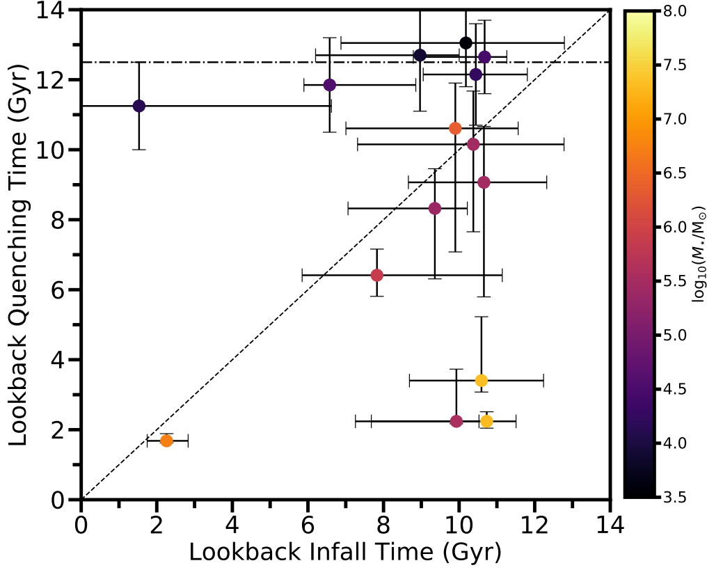
Figure 5.3: The relationship between quenching time ( t_{\text{quench}} ) and infall time ( t_{\text{infall}} ) for our primary sample of MW satellites. The points are color-coded by their present-day stellar mass, assuming M/L_V = 1 (see color bar for scale). The low-mass ( M_\star < 10^5 M_\odot ) satellites have quenching times consistent with suppression of star formation due to cosmic reionization, as illustrated by the dot-dashed line. For the “classical” ( M_\star = 10^5\text{--}8 M_\odot ) satellites, we generally find quenching and infall times that are consistent with a rapid cessation of star formation following accretion onto the MW. The lack of satellites with recent infall times is largely a consequence of observational bias, particularly at low stellar masses. Objects that recently fell onto the MW system preferentially reside at larger Galactocentric distances, such that we are likely “missing” a significant number of low-mass satellites for which we would infer more recent infall times. Finally, none of the satellites studied have quenching and infall times that strongly favor self-quenching via internal processes.
