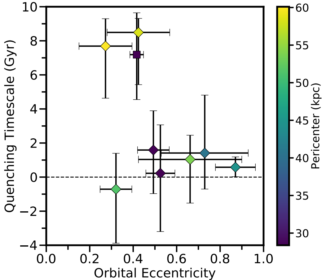
Figure 5.5: The quenching timescale as a function of orbital eccentricity, color-coded by pericentric distance, for the MW satellites with M_{\star} > 10^5 M_{\odot} in our primary sample. Due to the limitations of modeling Sag using the pELVIS simulations, it is given a different marker (square) to distinguish it from the other satellites (diamonds) in this analysis. The satellite galaxies with the longest quenching timescales are on orbits with some of the smallest eccentricities – i.e. more circular orbits. When combined with the relatively large pericentric distances for their orbits, these dwarf galaxies have likely experienced lower ram-pressure stripping, on average, allowing them to retain more of their cold gas reservoir and continue to form stars longer than satellites on more radial orbits.
