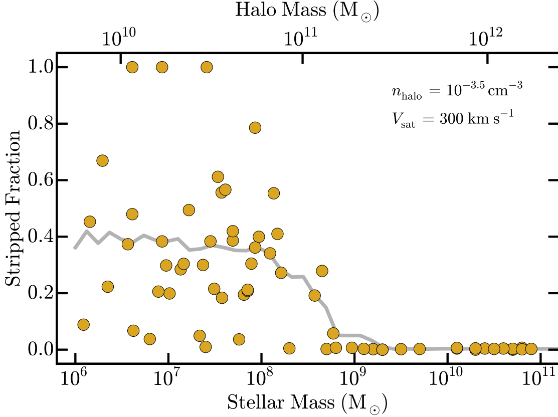
Figure 3.3: The fraction of H I gas stripped ( f_{\text{stripped}} ) via ram pressure as a function of stellar mass for our sample of 66 dwarf galaxies, assuming a host halo gas density of n_{\text{halo}} = 10^{-3.5} \text{ cm}^{-3} and a satellite velocity of V_{\text{sat}} = 300 \text{ km s}^{-1} . The grey solid line corresponds to the mean f_{\text{stripped}} computed in a sliding bin of width 0.6 dex in stellar mass. At stellar masses greater than roughly 10^9 M_{\odot} , we find that satellite systems are unaffected by ram pressure in a Milky Way-like environment. At M_{\star} \lesssim 10^{8.5} M_{\odot} , however, ram pressure is increasingly effective, with infalling systems typically having \sim 40\% of their cold gas stripped. It is worth noting that the scatter in the stripped fraction at fixed stellar mass is driven entirely by the variation in the H I surface density profiles. For reference, we include the corresponding halo mass for each system, as inferred via the stellar mass-halo mass relation of Garrison-Kimmel et al. (2014a).
