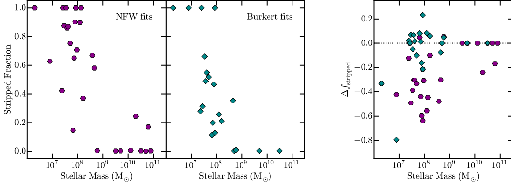
Figure 3.4: ( Left ): the fraction of HI gas ram-pressure stripped ( f_{\text{stripped}} ) as a function of stellar mass for the subset of systems with mass profiles determined via dynamical fits to an NFW profile (de Blok et al., 2008; Oh et al., 2015) and to a Burkert profile (Pace, 2016). As in Fig. 3.3, we assume a halo gas density of n_{\text{halo}} = 10^{-3.5} \text{ cm}^{-3} and a satellite velocity of V_{\text{sat}} = 300 \text{ km s}^{-1} . ( Right ): the difference in the fraction of HI gas stripped relative to the corresponding result (see Fig. 3.3) assuming our fiducial mass profile inferred via the stellar mass-halo mass relation of Garrison-Kimmel et al. (2014a): \Delta f_{\text{stripped}} = f_{\text{stripped, fid}} - f_{\text{stripped, dyn}} . In general, the mass profiles inferred from dynamical modeling favor cored halos, such that stripping is more efficient relative to our fiducial model. Moreover, while there is significant scatter from galaxy to galaxy based upon the assumed mass profile, the qualitative results are universal with ram-pressure stripping becoming increasingly effective at M_{\star} < 10^{8-9} M_{\odot} .
