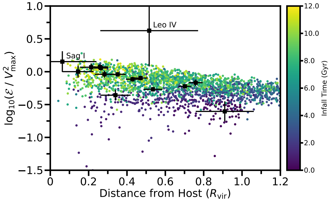
Figure 5.1: The binding energy ( \mathcal{E} ), scaled by the present-day V_{\text{max}} of the host, as a function of distance from the host (in units of host R_{\text{vir}} ) for subhalos in the pELVIS simulation suite. Each point is color-coded by the lookback time to first infall for the subhalo. The black squares correspond to the Milky Way satellites in our primary sample, assuming M_{\text{vir}} = 1.3 \times 10^{12} M_{\odot} , R_{\text{vir}} = 300 kpc, R_s = 18.75 kpc, and V_{\text{max}} = 200 km/s. To constrain t_{\text{infall}} , we select the 15 subhalos closest to each MW dwarf in the plotted parameter space, restricting to only those subhalos that also have the same directionality in their host-centric radial velocity component. The error bars illustrate the selection region for each MW dwarf based on this selection criteria (see §5.2 for more details). There exists a strong gradient in typical infall time within this parameter space. Many of the Milky Way satellites reside in regions with well-defined infall times, such that strong constraints can be placed on t_{\text{infall}} . Two objects, Sag I and Leo IV, are not well matched in this analysis, see §5.4 for a more detailed discussion.
