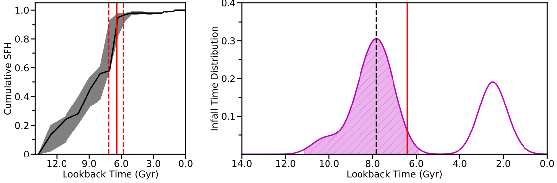
Figure 5.2: Illustrative example of both the quenching time and infall time measurements. Left: The cumulative SFH for Leo II, adapted from Weisz et al. (2014a), showing the adopted quenching time (solid red line) and corresponding 1\sigma uncertainty in the quenching time (dashed red lines). Right: The distribution of infall times for Leo II based on selecting the 15 subhalos that both reside nearest to Leo II in the \log(\mathcal{E}/V_{\text{max}}^2) –host-centric distance space (see Fig. 5.1) and have the same directionality in their radial velocity. The t_{\text{infall}} KDE (magenta line) is inferred using a gaussian kernel with a bandwidth selected via a leave-one-out cross validation grid search. We adopt the peak in the distribution (black dashed line) as the characteristic infall time for Leo II. The accompanying magenta shaded region illustrates the bounds on the uncertainty in the inferred t_{\text{infall}} , corresponding to the most probable region encompassing 68 % of the total distribution. For reference, the red line shows the quenching time as derived from the star formation history in the left panel. The typical Leo II-like subhalo in the simulations falls onto the host system for the first time \sim 2 Gyr prior to the cessation of star formation. This relatively fast quenching timescale is consistent with previous statistical work and favors ram-pressure stripping as the dominant quenching mechanism, perhaps assisted by tidal stripping and stellar feedback during pericentric passage.
