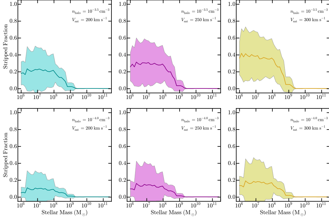
Figure 3.5: The fraction of HI gas stripped ( f_{\text{stripped}} ) via ram-pressure stripping as a function of satellite stellar mass for our sample of 66 dwarf galaxies. The solid line in each panel gives the mean f_{\text{stripped}} in a sliding bin of width 0.6 dex in stellar mass, with the shaded region tracing the corresponding 1\sigma scatter. In the top and bottom rows, we assume a host halo gas density of n_{\text{halo}} = 10^{-3.5} \text{ cm}^{-3} and 10^{-4.0} \text{ cm}^{-3} , respectively. From left to right , the satellite velocity varies from 200 (cyan) to 250 (magenta) to 300 \text{ km s}^{-1} (gold). While the efficiency of ram-pressure stripping depends on the assumed properties of the host halo, such that \langle f_{\text{stripped}} \rangle ranges from \sim 10 - 40\% , the satellite stellar mass where ram-pressure stripping becomes significant is universally < 10^9 M_{\odot} .
