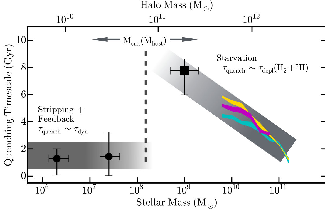
Figure 3.8: The dependence of the satellite quenching timescale on satellite stellar mass in Milky Way-like and more massive host halos ( > 10^{12} M_{\odot} ), as adapted from Fillingham et al. (2015). The magenta, gold, and cyan colored bands show the constraints from Wetzel et al. (2013) for satellites in host halos of M_{\text{host}} \sim 10^{12-13} M_{\odot} , 10^{13-14} M_{\odot} , 10^{14-15} M_{\odot} , respectively. The black square and circles correspond to the typical quenching timescale for intermediate- and low-mass satellites from Wheeler et al. (2014) and Fillingham et al. (2015), respectively. The light grey shaded regions highlight the expected dominant quenching mechanism as a function of satellite mass, while the vertical dashed black line denotes the critical mass scale below which satellite quenching becomes increasingly efficient. At M_{\star} \gtrsim 10^8 M_{\odot} , the satellite quenching timescales show broad agreement with the observed gas depletion timescales for field systems, suggesting that starvation is the main driver of satellite quenching at these masses. At low masses, stripping – potentially assisted by stellar feedback and a clumpy host CGM – is the most probable mechanism responsible for the high satellite quenched fractions and short quenching timescales observed in the Local Group. The critical satellite stellar mass, M_{\text{crit}} , at which the dominant quenching mechanism shifts from starvation to stripping should depend on the halo mass of the host system, with more massive hosts able to strip more massive satellites.
