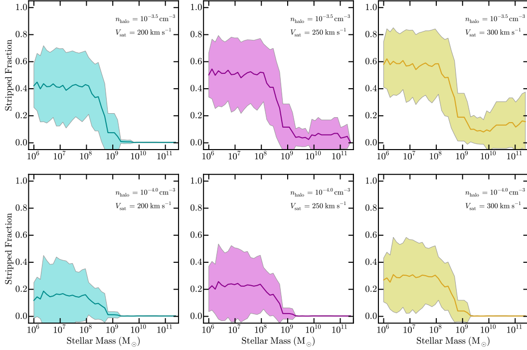
Figure 3.6: The fraction of H I gas stripped ( f_{\text{stripped}} ) via ram-pressure and turbulent viscous stripping as a function of satellite stellar mass for our sample of 66 dwarf galaxies. The solid line in each panel gives the mean f_{\text{stripped}} in a sliding bin of width 0.6 dex in stellar mass, with the shaded region tracing the corresponding 1\sigma scatter. In the top and bottom rows, we assume a host halo gas density of n_{\text{halo}} = 10^{-3.5} \text{ cm}^{-3} and 10^{-4.0} \text{ cm}^{-3} , respectively. From left to right , the satellite velocity varies from 200 (cyan) to 250 (magenta) to 300 \text{km s}^{-1} (gold). Including both ram-pressure and turbulent viscous stripping, we find an increase in the fraction of stripped gas, such that the majority of gas is removed from low-mass satellites orbiting hosts with a halo gas density of 10^{-3.5} \text{ cm}^{-3} .
