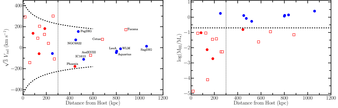
Figure 4.1: Left : Host-centric radial velocity (scaled by \sqrt{3} to approximately account for tangential motion) for all known Local Volume dwarf galaxies in the stellar mass range 10^6 - 10^8 M_{\odot} as a function of distance from the nearest host (either the Milky Way or M31). The dotted vertical line roughly corresponds to the virial radius of a Milky Way-like host and the dashed lines correspond to the boundary between bound and unbound systems. Satellite points are color-coded according to their observed H I gas fraction, with blue (and red) points denoting gas-rich (and gas-poor) systems, respectively. The closed points signify H I detections, while the open points correspond to upper limits on the total H I mass. Right : The gas fraction ( M_{\text{HI}}/M_* ) as a function of distance from the nearest host for the same dwarf galaxies as in the left panel. The horizontal dashed line corresponds to a gas fraction of 0.2, below which systems are considered quenched.
