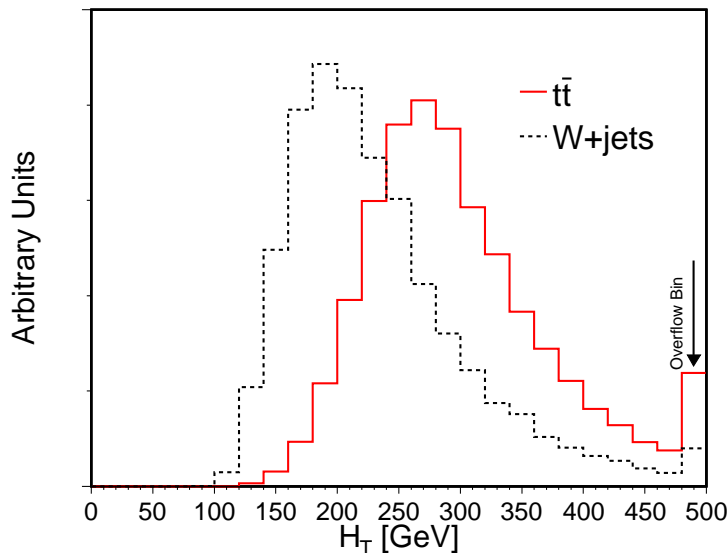
FIG. 2: H_T distributions, normalized to unity, for t\bar{t} (solid line) and W +jets (dotted line) PYTHIA Monte Carlo events with three or more jets after the event selection described in the text.
