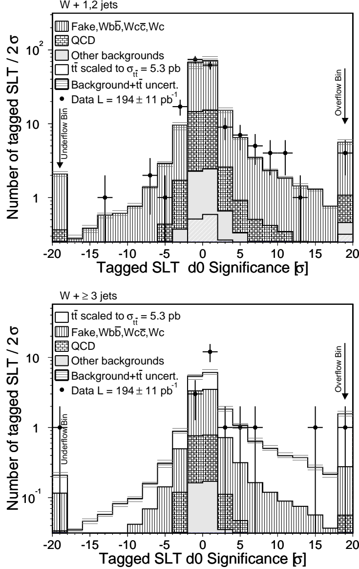
FIG. 17: The impact parameter ( d_0 ) significance for tagged events, compared with expectations from backgrounds plus t\bar{t} . The upper plot is for W+1 and 2 jet events and the lower plot for W+\geq 3 jet events.
