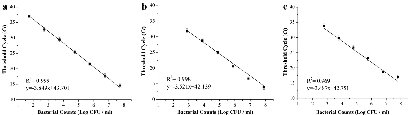
FIG 2 Quantification standard curves targeting thh (a), tdh (b), and trh (c) genes in V. parahaemolyticus .
