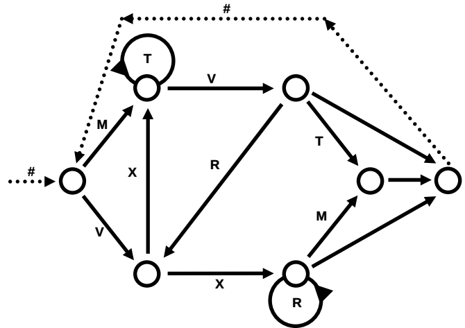
Figure 1: The transition graph representation of RM1 corresponding to the Reber grammar.
