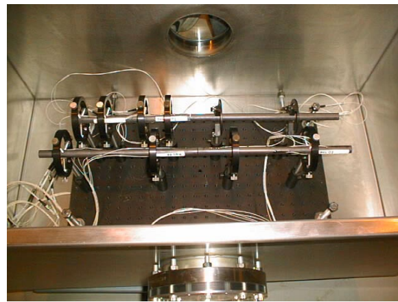
Figure 2: Carbon target rod mounted in E951 target box.
