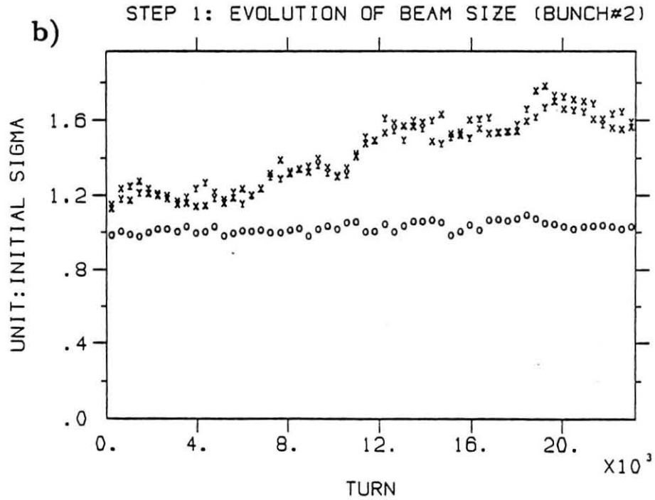
Figure 2: The time evolution of beam sizes of (a) Beam+ and (b) Beam-, respectively, for \epsilon^- = 81.76 nm·rad, up to 24000 turns. The points x, y and o represent the horizontal, vertical, and longitudinal beam sizes, respectively, in units of their nominal rms sizes.
