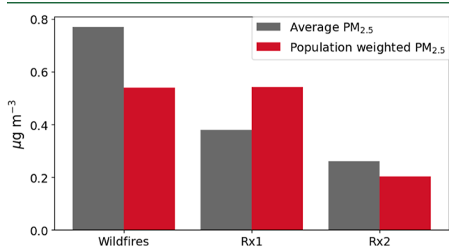
Figure 5. Modeled annual average surface fire-derived PM_{2.5} concentrations and population-weighted PM_{2.5} across the study area under the wildfire and Rx1 and Rx2 scenarios.
