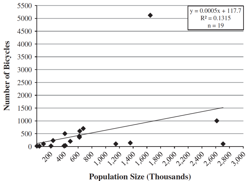
Fig. 5. Comparison of system size versus population size in North America. Source of city size data: U.S. Census (2010) and Can Stat (2011).
