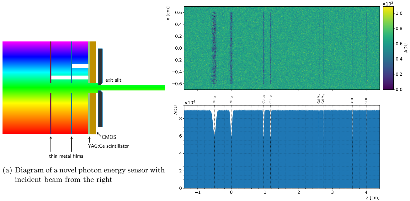
(b) Toy simulation of the photon energy sensor where x corresponds to the horizontal position and z corresponds to the vertical position on the CMOS image sensor. The intensity reductions are modeled using Gaussian distributions with widths of 1 eV.
