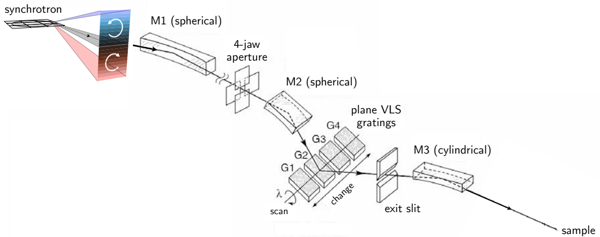
Figure 3: Diagram of Beamline 6.3.1, a bending magnet beam line that is primary used for X-ray magnetic circular dichroism spectroscopy at the Advanced Light Source (figure adapted from Ref. 10). The beam line optics consist of a horizontal focusing concave spherical mirror (M1), a 4-jaw aperture, a vertical focusing concave spherical mirror (M2), interchangeable planar VLS gratings, an exit slit, and a vertical focusing mirror (M3).
