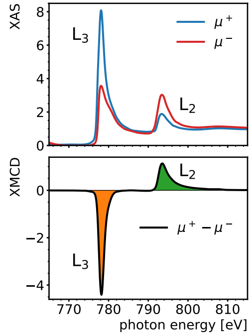
(b) X-ray absorption (top) and X-ray magnetic circular dichroism (bottom) spectra for the Co L_3 and L_2 edges (figure adapted from Ref. 4)
