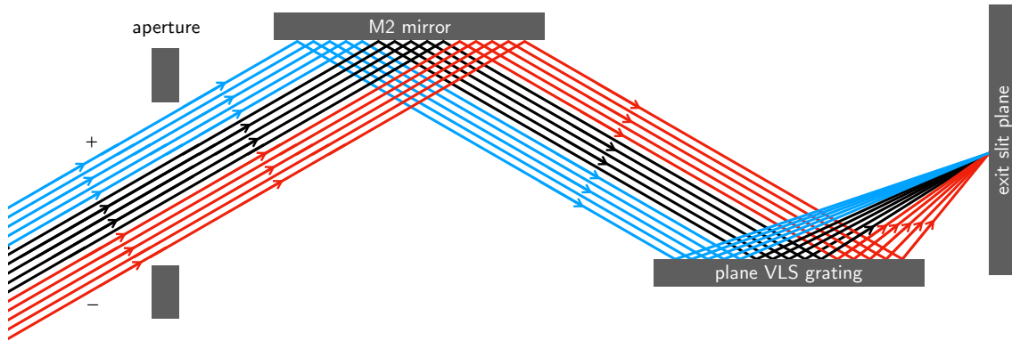
(c) Diagram of X-rays of linear and circular polarizations passing through a variable-line-spacing (VLS) plane grating monochromator
