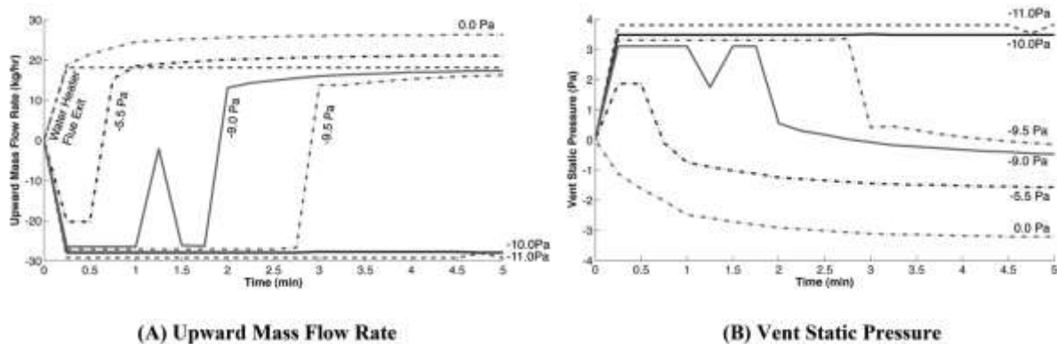
Figure 10: VENT-II predicted that the orphaned water heater located in Stockton, CA will spill (A) and backdraft (B) for the duration of the test (5 minutes) when the CAZ pressure, with respect to outdoors, is less than or equal to -10.0 Pa (-0.040 in.w.c.).
