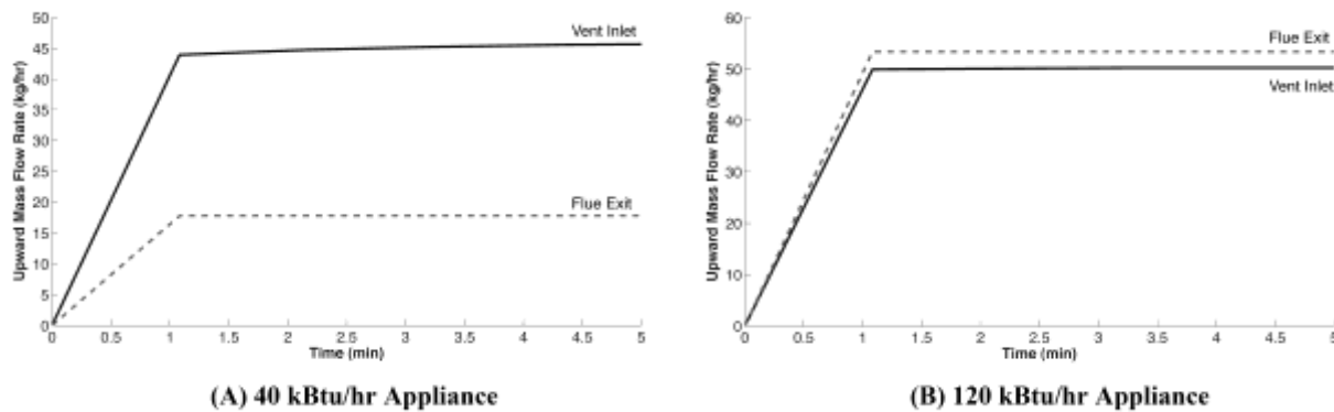
Figure 2: For a 40 kBtu/hr appliance with an appropriately sized vent system (A), the mass flow rate of gases at the flue outlet is less than the mass flow rate of gases in the vent, which indicates that dilution air is entering the vent and the appliance is not spilling. However, for an oversized 120 kBtu/hr (35.2 kW) appliance using the same vent system sized for a 40 kBtu/hr (11.7 kW) appliance (B), the mass flow rate of gases at the flue outlet is greater than the mass flow rate of gases in the vent, which indicates that the appliance is spilling.
