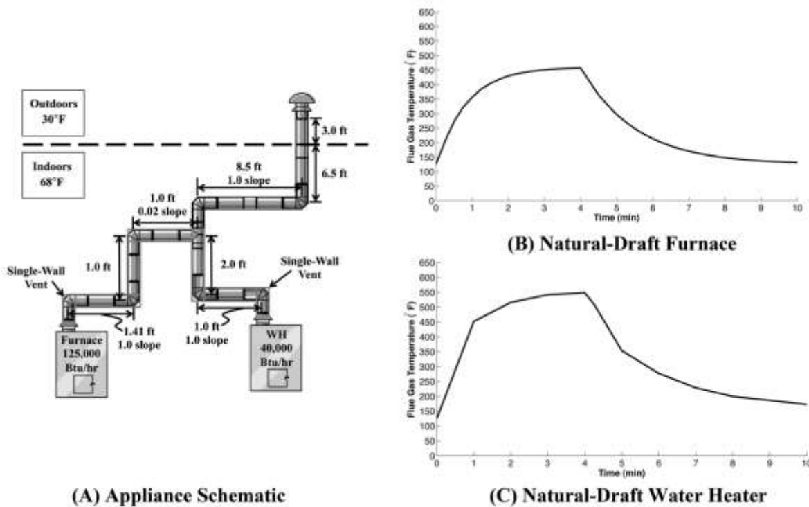
Figure 3: Schematic of furnace and water heater vent system in Twin Cities, MN as modeled in VENT-II (A) and the simulated flue gas temperature for the furnace (B) and the water heater (C) during one operating cycle. The furnace vent connector is composed of two, 6 in. (15.24 cm) diameter single-walled vents. The water heater (WH) vent is composed of two circular, 4 in. (10.16 cm) diameter single-walled vents. The common vent contains four circular, 6 in. (15.24 cm) diameter B-vents. Horizontal sections with slopes greater than or equal to 1.0 are assumed to have 45-degree elbows. Horizontal sections with slopes less than 1.0 are assumed to have 90-degree elbows.
