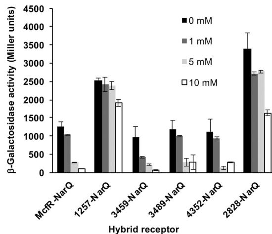
FIG 8 \Phi ( narG-lacZ ) expression in E. coli VJS5054 carrying six different MCP-NarQ hybrid receptors in response to propionate. \beta -Galactosidase assays were carried out on cultures grown with the indicated concentrations of propionate. Results are averages from at least three independent experiments, with error bars representing standard deviations.
