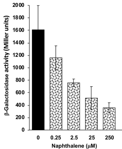
FIG 7 \Phi ( narG-lacZ ) expression in E. coli VJS5054 carrying the NahY-NarQ hybrid reporter. \beta -Galactosidase assays were carried out on cultures grown with the indicated concentrations of naphthalene. Results are averages from at least three independent experiments, with error bars representing standard deviations.
