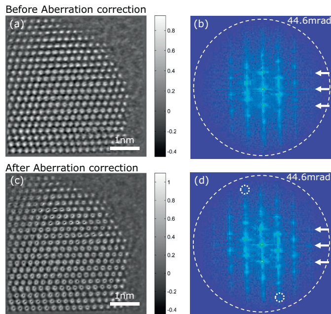
Fig. 4. The phase image of the complex transmission function reconstructed using ptychography WDD (a) before and (c) after post-acquisition aberration correction. The Fourier transform of the complex phase images are shown in (b) and (d), respectively. The arrows point to diffraction spots that are not visible before aberration correction, but become visible after aberration correction. The 442 diffraction spots indicated by the small dashed circles in (d) corresponds to a reciprocal scattering angle of 39 mrad and a real space spacing of 0.68 Å. The big dashed circles indicates the diffraction limited resolution of 44.6 mrad, which is twice the convergence semi-angle of the probe forming aperture. The diffraction patterns were recorded using 66 \times 264 detector pixels at 4000 frames per second speed.
