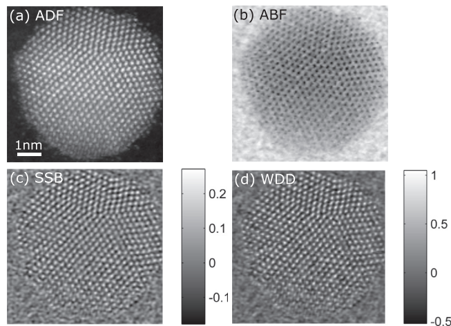
Fig. 3. Imaging a gold nanoparticle on a thin carbon support using (a) simultaneous ADF, (b) synthetic ABF, ptychography SSB phase and WDD phase. Colorbar in (c,d) in unit of radian. The synthetic ABF has a collection angle of 7.2–14.4 mrad in (b). The diffraction patterns were recorded using 264 \times 264 detector pixels at 1000 frames per second speed.
