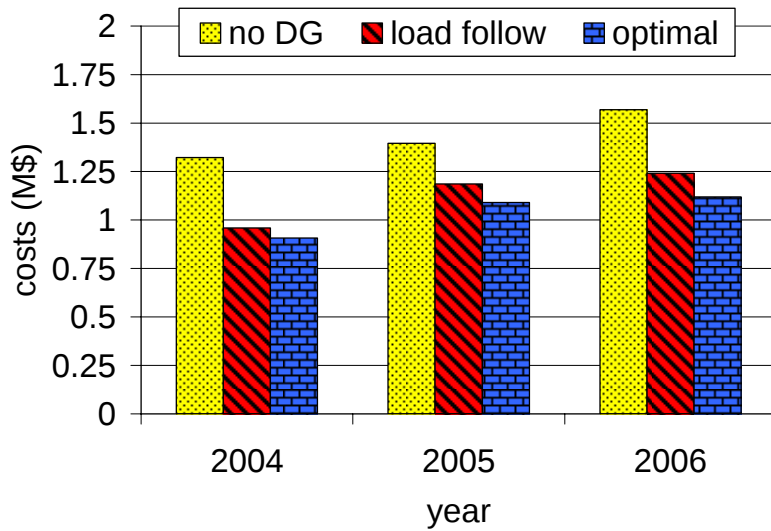
Figure 14. annual energy costs under RTP tariff and three control strategies
