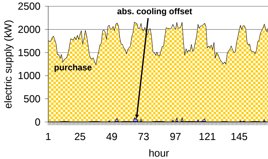
Figure 22. optimal electric supply under TOU tariff for the first full week of November 2005
