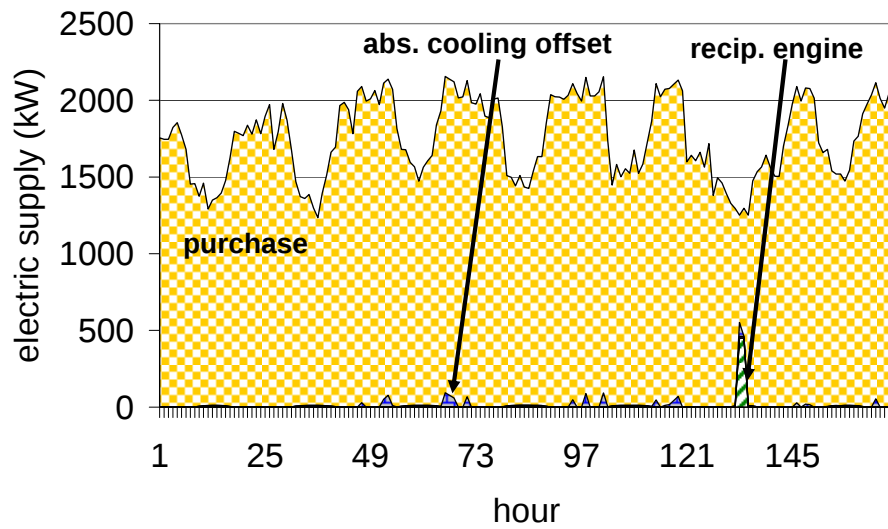
Figure 23. optimal electric supply under CPP tariff for the first full week of November 2005
