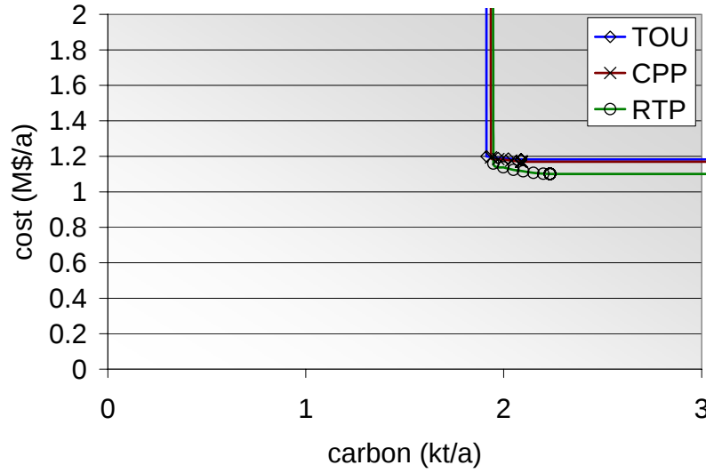
Figure 28. cost/carbon Pareto curve
