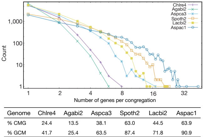
Figure S1 Extent of overlapping transcription. Top: distribution of number of genes per congregation. Both axes are in log scale. The bottom part summaries the percentage of congregations with more than one gene (% CMG) and percentage of genes belong to congregations with two or more genes (% GCM).
