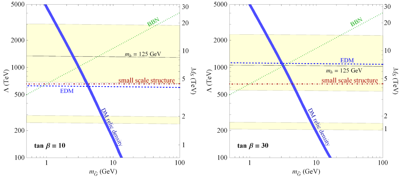
FIG. 4 (color online). Summary plot of all constraints on the minimal GMSB scenario in the (m_{\tilde{G}}, \Lambda) plane for \tan\beta = 10 (left) and 30 (right), N_S = 1 , and \mu > 0 . The Higgs mass is in the allowed range in the light-yellow-shaded regions, and \Omega_{\tilde{G}}h^2 = 0.112 \pm 0.006 in the dark-blue-shaded bands. The EDM constraint (for \tan\theta_{CP} = 0.1 ) and BBN constraint ( \tau_\chi < 1 s) exclude parameter space below the indicated contours, and small-scale structure ( \lambda_{FS} \lesssim 0.5 Mpc) favors parameter space above or near the indicated contour. The stop mass parameter M_S is largely determined by \Lambda and insensitive to m_{\tilde{G}} in the range plotted, and it is given on the right-hand axis.
