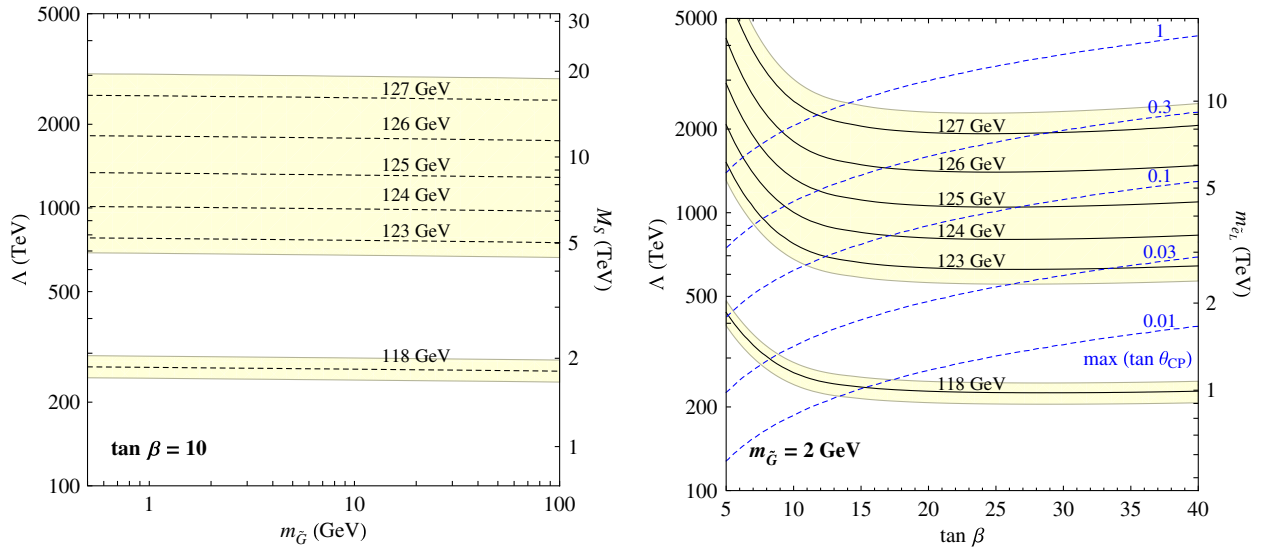
FIG. 1 (color online). Left : Contours of constant Higgs boson mass in minimal GMSB in the (m_{\tilde{G}}, \Lambda) plane for \tan\beta = 10 , N_5 = 1 , and \mu > 0 . The yellow-shaded regions are the allowed ranges for the Higgs boson mass, given the recent exclusions from the LHC. The stop mass parameter M_S is largely determined by \Lambda and insensitive to m_{\tilde{G}} in the range plotted, and it is given on the right-hand axis. Right : Dashed blue contours of constant maximal \tan\theta_{CP} allowed by the upper bound on the electron EDM in the (\tan\beta, \Lambda) plane for m_{\tilde{G}} = 2 GeV, N_5 = 1 , and \mu > 0 . The preferred Higgs mass regions are as in the left panel. The left-handed selectron mass m_{\tilde{e}_L} is largely determined by \Lambda and insensitive to \tan\beta , and it is given on the right-hand axis.
