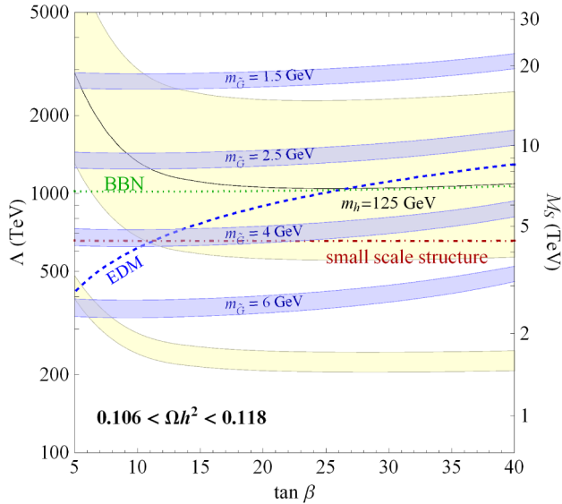
FIG. 5 (color online). Summary plot of all constraints on the minimal GMSB model in the (\tan\beta, \Lambda) plane for N_5 = 1 , \mu > 0 . The blue-shaded bands correspond to regions where the correct gravitino relic density is achieved for the indicated gravitino mass. Constraints from EDMs, BBN, small-scale structure, and the Higgs boson mass are as in Fig. 4. The stop mass parameter M_S is largely determined by \Lambda and insensitive to \tan\beta , and it is given on the right-hand axis.
