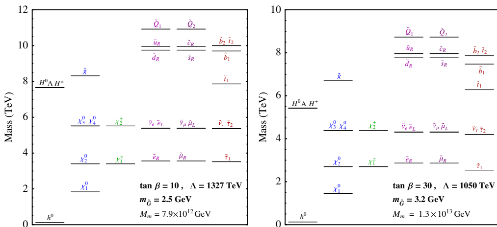
FIG. 6 (color online). Superpartner mass spectra for example models with \tan\beta = 10 (left) and 30 (right), \Lambda , m_{\tilde{G}} and M_m as indicated, and N_5 = 1 and \mu > 0 . For each case, the parameters \Lambda and M_m have been uniquely fixed by requiring that m_h = 125 GeV and \Omega_{\tilde{G}} = 0.112 . For the \tan\beta = 10 example, \tau_\chi = 0.18 s, \lambda_{FS} = 0.19 Mpc, and \max(\tan\theta_{CP}) = 0.43 . For the \tan\beta = 30 example, \tau_\chi = 0.92 s, \lambda_{FS} = 0.27 Mpc, and \max(\tan\theta_{CP}) = 0.090 .
