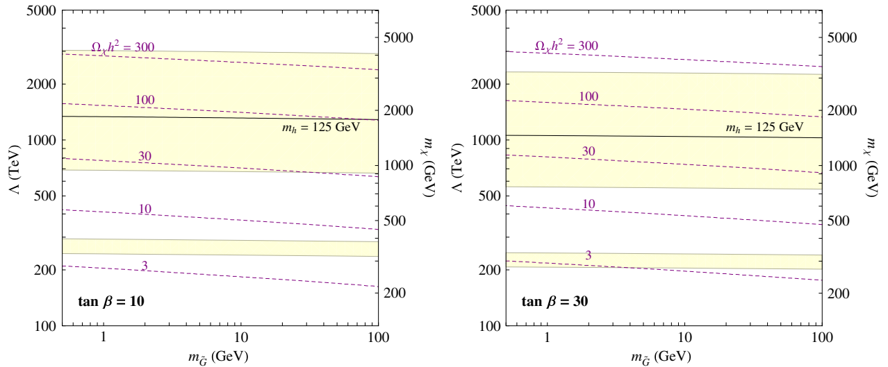
FIG. 2 (color online). Contours of constant neutralino relic density (dashed, purple) for \tan\beta = 10 (left) and 30 (right), N_5 = 1 , and \mu > 0 , computed with MICROMEAS. The preferred Higgs mass regions from Fig. 1 are also shown. The neutralino mass m_\chi is largely determined by \Lambda and insensitive to m_{\tilde{G}} in the range plotted, and it is given on the right-hand axis.
