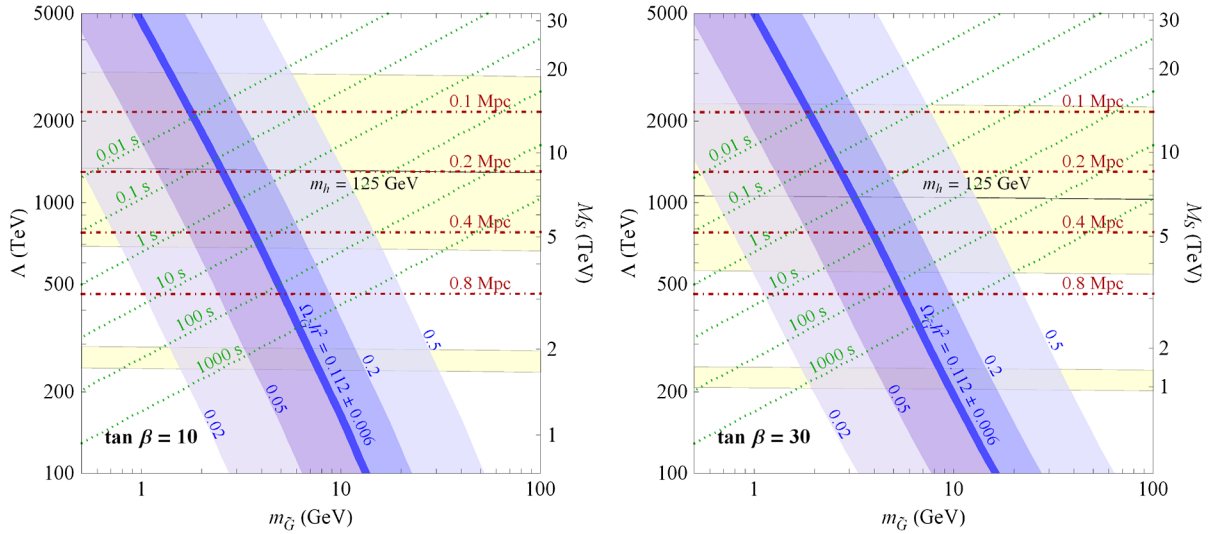
FIG. 3 (color online). Contours of constant gravitino relic density (blue, shaded), neutralino lifetime (dotted, green) and free-streaming length (dot-dashed, red) for \tan\beta = 10 (left) and 30 (right), N_5 = 1 , and \mu > 0 . The preferred Higgs mass regions from Fig. 1 are also shown. The stop mass parameter M_S is largely determined by \Lambda and insensitive to m_{\tilde{G}} in the range plotted, and it is given on the right-hand axis.
