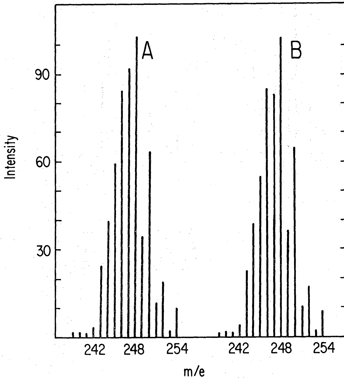
Fig. 4. The calculated (A) and observed (B) mass spectral bands for the species \text{SnH}_n^+ ; n = 0, 1, 2, \text{ or } 3 . The fragmentation pattern is A_0 = 0.300 , A_1 = 0.330 , A_2 = 0.067 , and A_3 = 0.300 , and was calculated from the intensities of peaks at m/e = 251, 252, 253, \text{ and } 254 .
