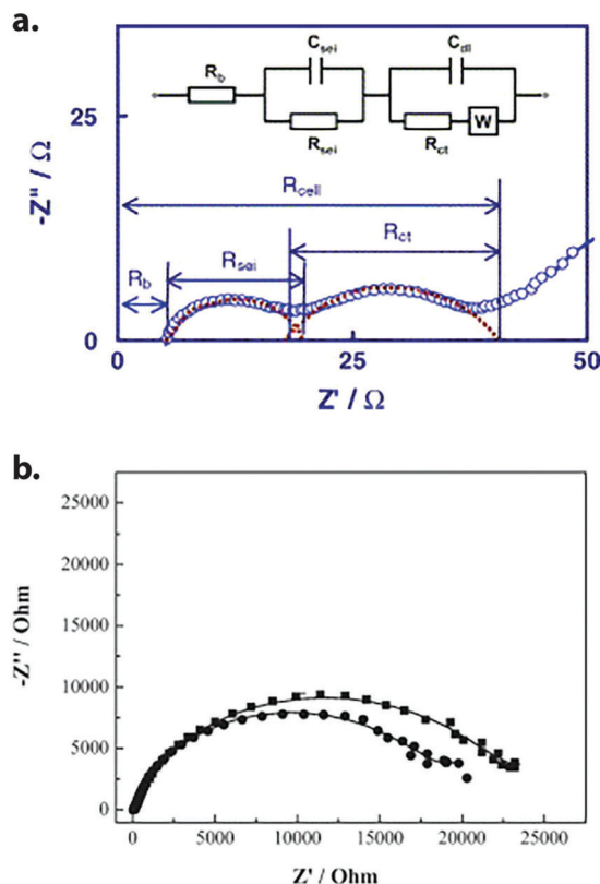
Fig. 6 (a) Nyquist plot of Li-ion cell impedance showing relatively well-separated semicircles. In this case, both the individual values of R_{\text{SEI}} and R_{\text{ct}} can be reasonably determined (although they each represent lumped values for cathode and anode processes). Reprinted from ref. 31 with permission from Elsevier. (b) Nyquist plot of Li||MCMB half-cell impedance, where only one semicircle is distinguishable. In this case R_{\text{SEI}} cannot be separated from R_{\text{ct}} , either due to similar time constants for both processes or because one is much larger than the other. Additional context is required to interpret the combined “interfacial resistance.” Reprinted from ref. 66 with permission from Elsevier.
