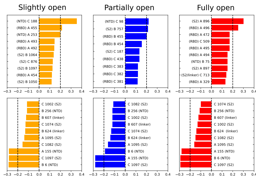
Fig. 5. Residues with large changes in normalized BC due to RBD opening. (Upper) Largest positive changes; (Lower) negative changes; chain index (A, B, or C) mentioned before the residue number. The location of the residue (NTD, RBD, linker, or S2) is also mentioned next to the residue number.
