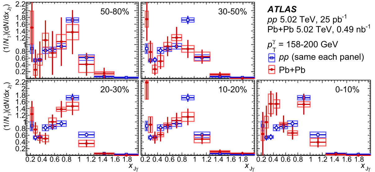
Fig. 7. Photon-jet p_T -balance distributions (1/N_\gamma)(dN/dx_{j\gamma}) in Pb + Pb events (red circles) with each panel showing a different centrality selection compared to that in pp events (blue squares). These panels show results for p_T^\gamma = 158-200 GeV. Total systematic uncertainties are shown as boxes, while statistical uncertainties are shown as vertical bars.
