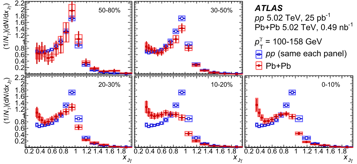
Fig. 6. Photon-jet p_T -balance distributions (1/N_\gamma)(dN/dx_{j\gamma}) in Pb + Pb events (red circles) with each panel showing a different centrality selection compared to that in pp events (blue squares). These panels show results for p_T^\gamma = 100-158 GeV. Total systematic uncertainties are shown as boxes, while statistical uncertainties are shown as vertical bars.
