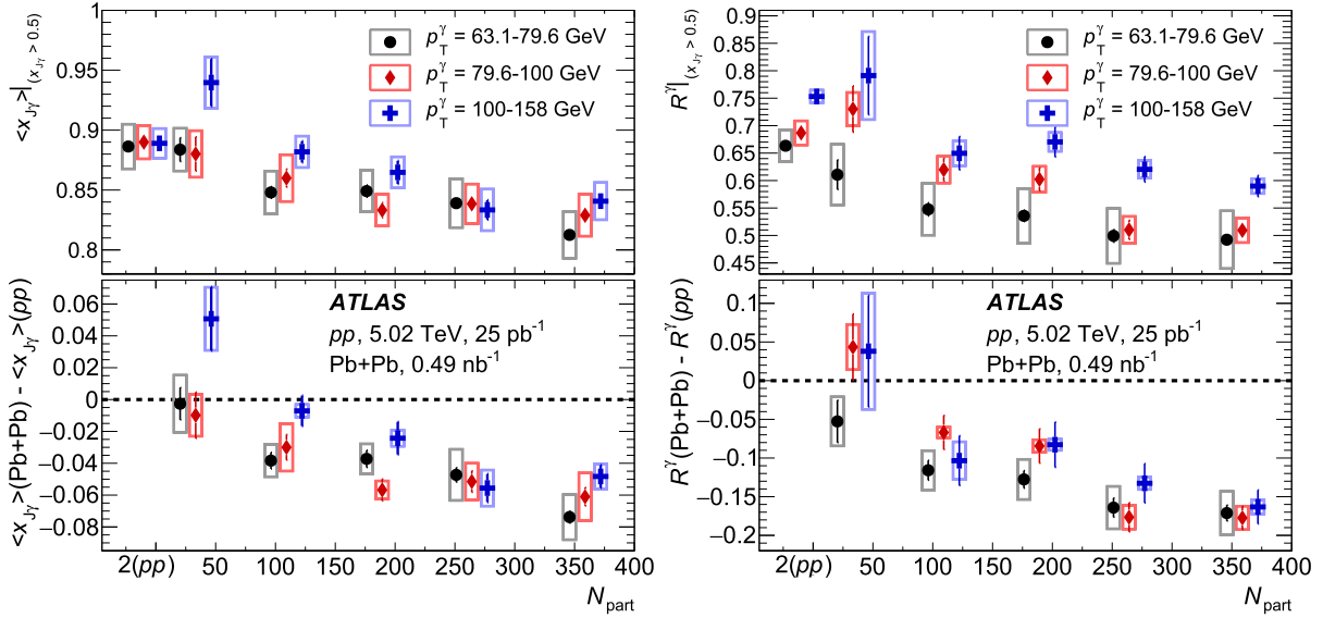
Fig. 8. Summary of (left) the mean jet-to-photon p_T ratio \langle x_{J\gamma} \rangle and (right) the total per-photon jet yield R^Y , calculated in the region x_{J\gamma} > 0.5 . The values are presented as a function of the mean number of participating nucleons N_{\text{part}} in top panels. Each colour and symbol represents a different p_T^Y interval, where the lowest and highest intervals are displaced horizontally for clarity. The points plotted at N_{\text{part}} = 2 correspond to pp collisions. The bottom panels show the difference between the Pb + Pb centrality selection and pp collisions. Boxes show the total systematic uncertainty while the vertical bars represent statistical uncertainties.
