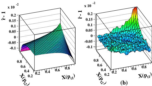
FIG. 4: Left: pair-density net ratio r_{model}[X(p_{t1}), X(p_{t2})] - 1 for model fit to mid-central (b) Au-Au collisions. Right: residuals (data - model) for mid-central collisions.
