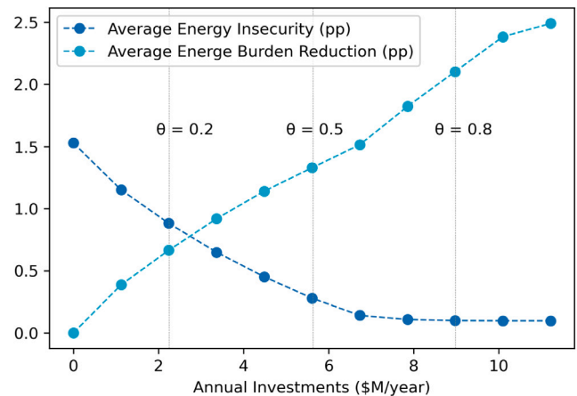
Fig. 3. Pareto front of energy insecurity as a function of the intervention costs. Comparison with the energy burden reduction for the same values of \theta .
