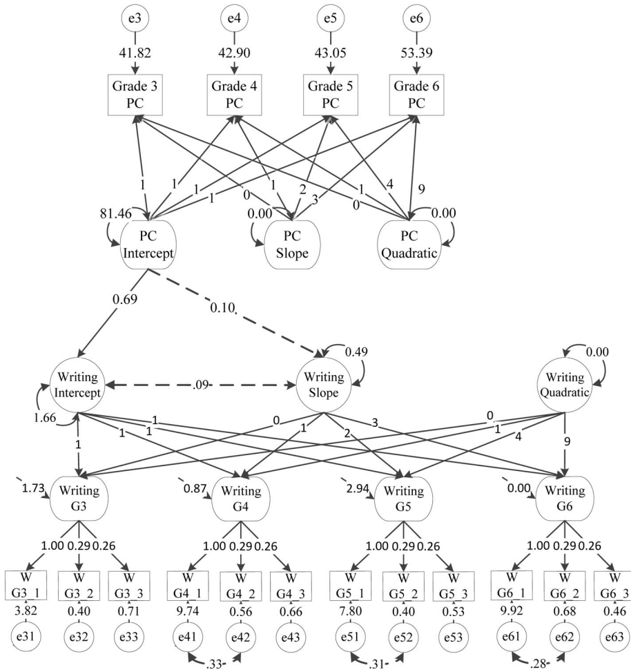
Figure 3. Latent reading comprehension development predicting latent writing development. PC = Passage Comprehension; W = Writing quality
