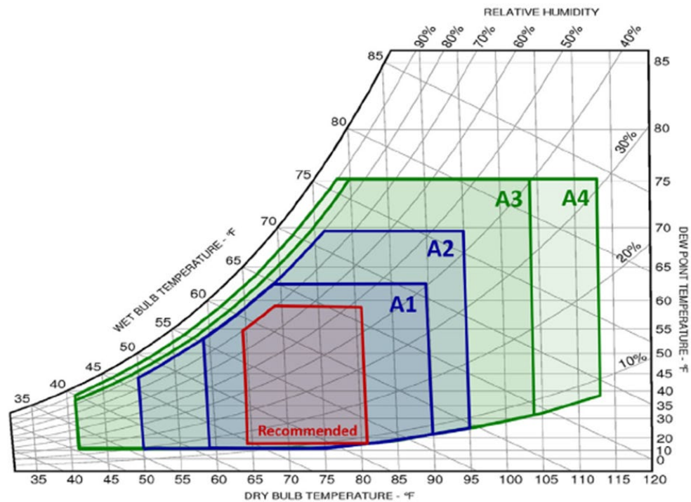
Figure 4. ASHRAE environmental envelopes (low level of pollutants in the data center).
